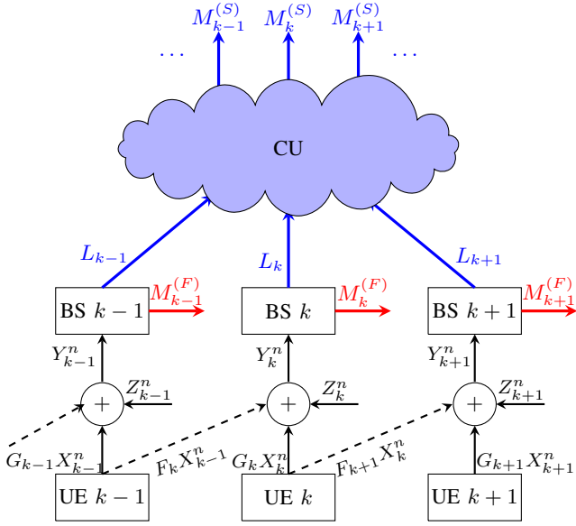
Fig. 1. System model
