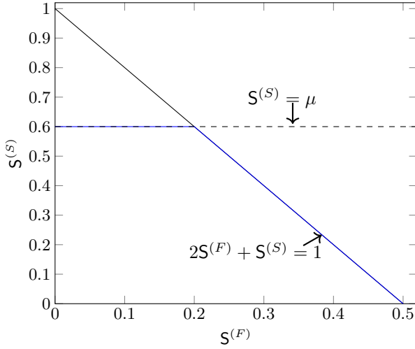
Fig. 3. Region S^*(\mu) for \mu = 0.6 in blue and \mu \geq 1 in black.
