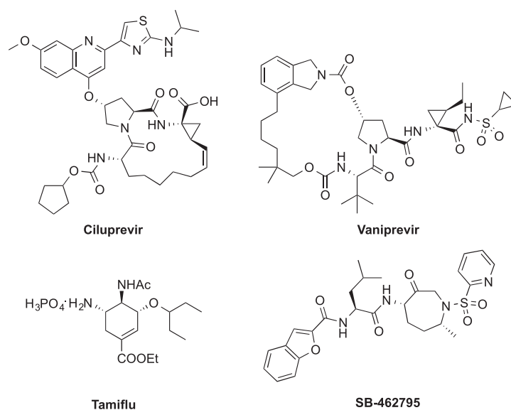
Fig. 1. Selected biologically active compounds obtained via RCM method.
