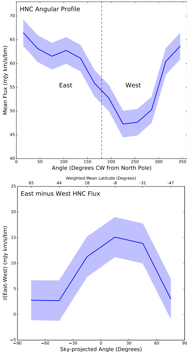
FIG. 5.— Top: Average radial HNC flux as a function of angle from Titan’s sky-projected north polar axis. Dashed line indicates 180^\circ ( i.e. the south pole). Bottom: Flux difference (east minus west) for HNC, as a function of angle from the bisector of Titan’s sky-projected polar axis, demonstrating a clear east-west asymmetry.
