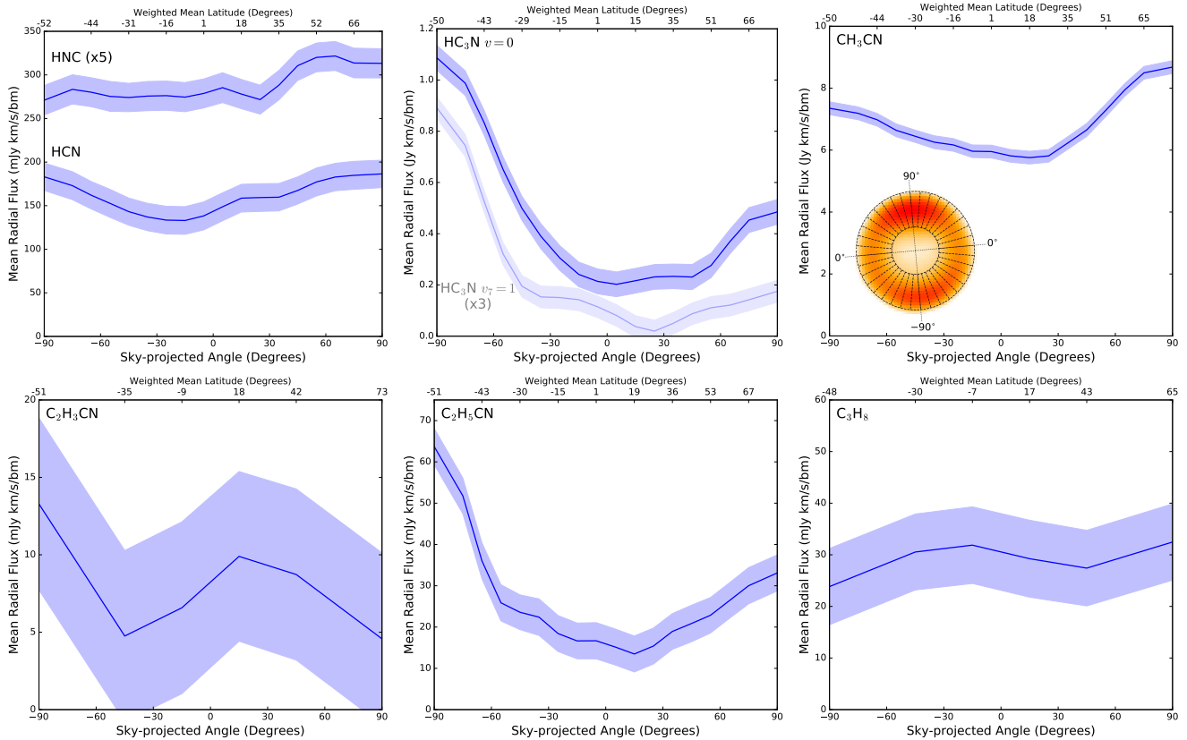
FIG. 4.— ALMA fluxes (radially averaged) as a function of angle from the bisector of Titan’s sky-projected polar axis — the coordinate system and angular binning scheme are indicated by the inset in the upper-right panel. Blue envelopes show the \pm 1\sigma error range. The weighted mean latitudes for each measurement are shown on the upper abscissa axes. HCN and HNC are shown in the same panel for comparison (with the HNC profile multiplied by 5 for display); similarly, the \text{HC}_3\text{N } \nu_7 = 1 profile is shown in a lighter colour (multiplied by a factor of 3), for comparison with \text{HC}_3\text{N } \nu = 0 .
