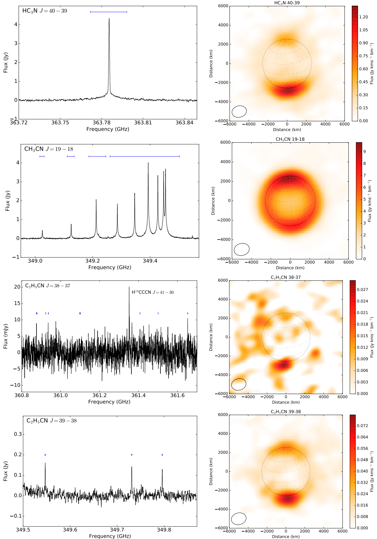
FIG. 1.— Continuum-subtracted molecular spectra and integrated emission maps for \text{HC}_3\text{N} , \text{CH}_3\text{CN} , \text{C}_2\text{H}_3\text{CN} and \text{C}_2\text{H}_5\text{CN} , observed using ALMA in 2017 May. Spectra (apart from \text{C}_2\text{H}_3\text{CN} ) were integrated over a circular aperture with radius 4300 km, centered on Titan. The \text{C}_2\text{H}_3\text{CN} spectrum was extracted from a beam centered at the S-polar emission peak for that molecule. Spectral integration range(s) for the emission maps are shown with blue bars. The grey wireframe spheres indicate Titan's surface and alignment in the field of view. Ellipse (lower-left) shows the spatial resolution (beam FWHM) for each map.
