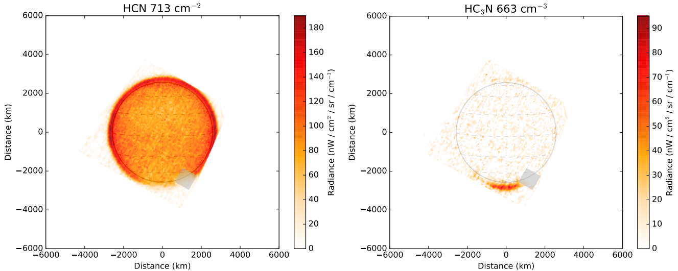
FIG. 3.— Cassini CIRS pushbroom maps of (continuum subtracted) HCN and \text{HC}_3\text{N} emission from Titan, obtained during the 2017-05-24 flyby (Cassini orbit #275). Image frequencies are given for each molecule. Grey boxes indicate missing data.
