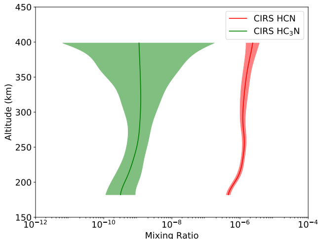
FIG. 7.— Cassini CIRS limb abundances for HCN and HC 3 N, retrieved at latitude -11^\circ .
