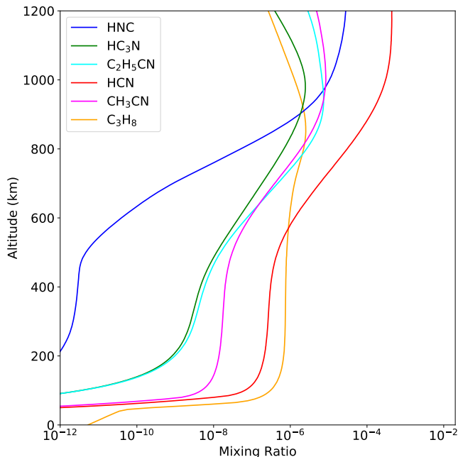
FIG. 8.— Predicted equatorial abundances as a function of altitude, from the recent photochemical model of Vuitton et al. (2019). The C_2H_5CN and HC_3N models include loss via sticking to aerosols.
