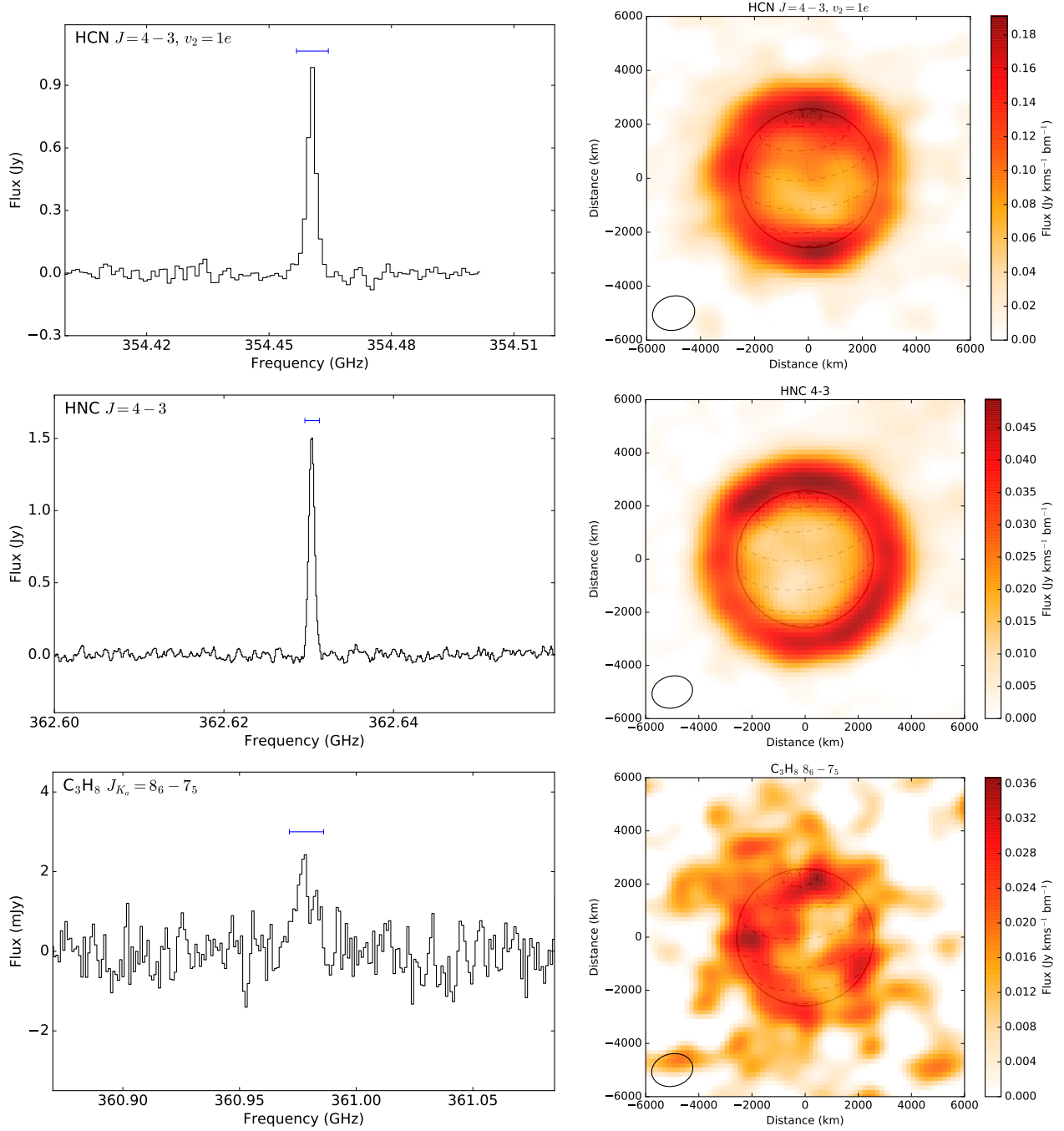
FIG. 2.— Same as Figure 1 but for HCN, HNC and C_3H_8 .
