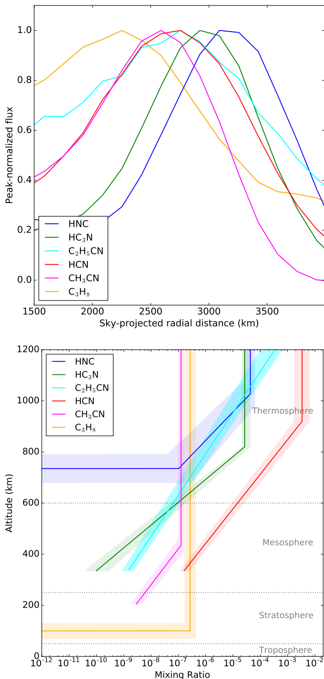
FIG. 6.— Top panel: Peak-normalized equatorial limb flux profiles observed using ALMA (excluding the regions within \pm 45^\circ of Titan’s north and south poles). Distances are with respect to the center of Titan’s disk, projected in the plane of the sky. Bottom panel: Retrieved vertical abundance profiles with 1\sigma error envelopes.
