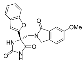
Figure 5. Hydantoin SCH900567.
