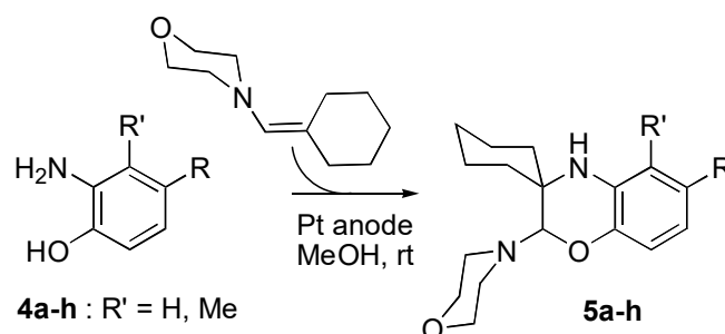
Scheme 2. Tandem Oxidation-IEDDA Reaction leading to 2-alkylamino-1,4-benzoxazine derivatives 5a-h
