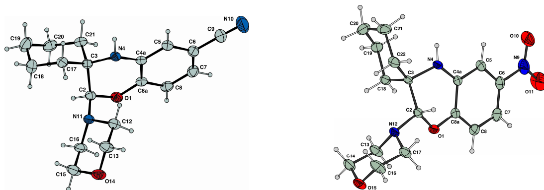
Figure 6. ORTEP view of 5e and 5f . Displacement ellipsoids are drawn at the 30% probability level.
