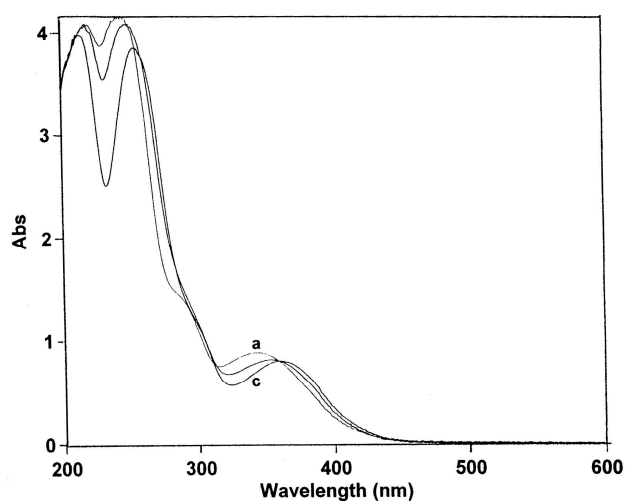
Figure 5. Spectrophotometric changes accompanying the electrochemical oxidation of 4a (2 mM) at a platinum anode ( E = +450 mV vs SCE), in deaerated MeOH containing tetraethylammonium hexafluorophosphate (20 mM), 4-cyclohexylidenemethylmorpholine (10 mM) and morpholine (2 mM): (a) 0 (before electrolysis); (b) 1; (c) 2.2 mol of electrons. Cell thickness, 0.1 cm.
