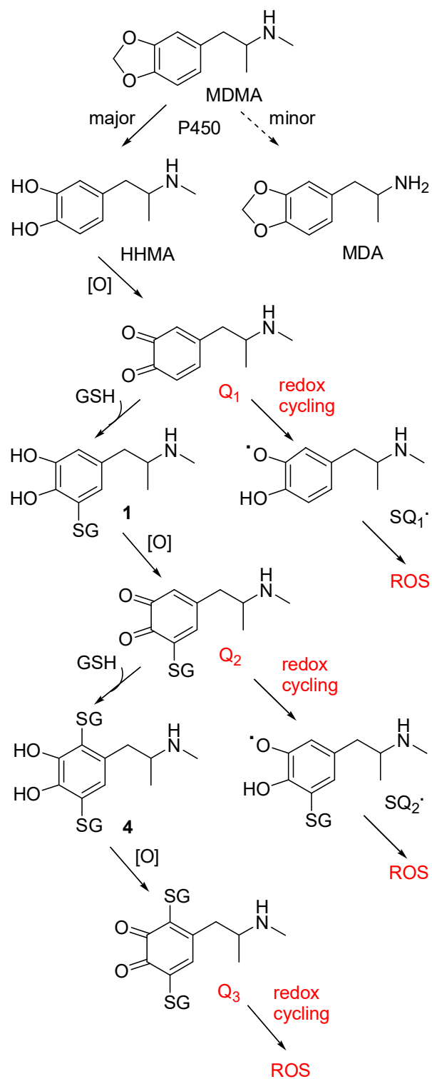
Scheme 1. Proposed Routes for MDMA Metabolism to Redox Active Catechol-Thioether Conjugates in Humans
