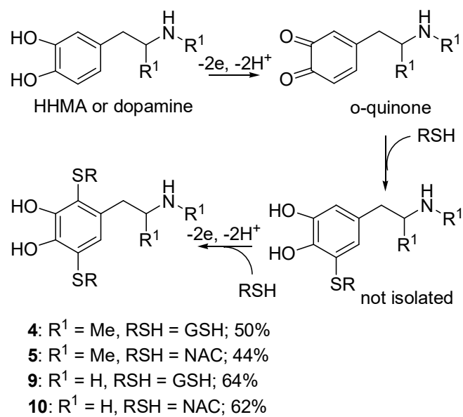
Scheme 2. Two-Step One-Pot Electrochemical Synthesis of bis-Catechol-Thioether Conjugates 4 , 5 , 9 and 10 .
