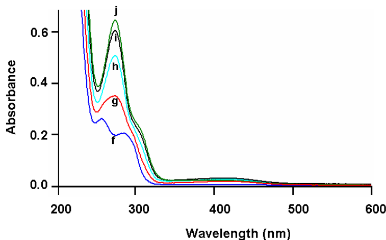
Figure 3. Spectrophotometric changes accompanying the multi-step one-pot electrosynthesis of S -(+)-catechol-thioether bis-conjugate 12 . (spectrum f ): after addition of 3 equiv of N -acetylcysteine to the two electron-oxidized solution of S -(+)-HHMA (1 mM), at a platinum anode ( E = +1.0 V versus Ag/AgCl), in deaerated 0.2 M HCl aqueous solution; (spectra g-j ): spectra recorded after the consumption of additional 3.5 mol of electrons: ( g ) 1.0, ( h ) 2.0, ( i ) 3.0, ( j ) 3.5 (end of the process). Cell thickness is 0.1 cm.
