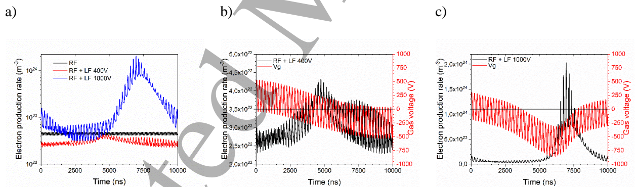
Figure 10. Time evolution of the electron production rate over half a LF cycle (a) for the RF-DBD, the DF-DBD in mode 1 and the DF-DBD in mode 2. Comparisons of gas voltage and electron production for (b) DF mode 1 and (c) DF mode 2.
