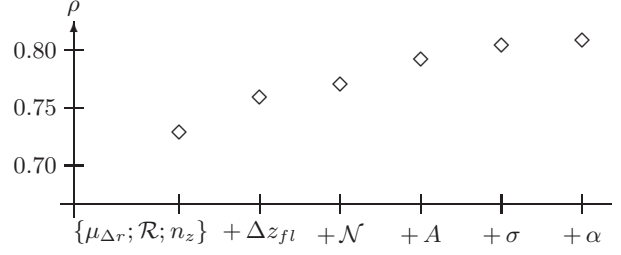
Figure 3: Overall Accuracy evolution depending on the features included in the SVM algorithm. Starting from the vector \{\mu_{\Delta r}; \mathcal{R}; n_z\} , the other ones are added progressively (Biberach area).
