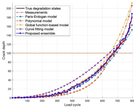
FIGURE 5. Degradation state estimation for the considered degradation trajectory using the proposed ensemble.
