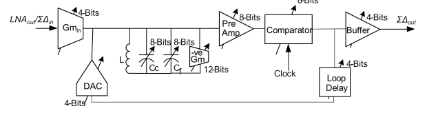
Fig. 6. Architecture of tunable BP RF \Sigma\Delta modulator.
