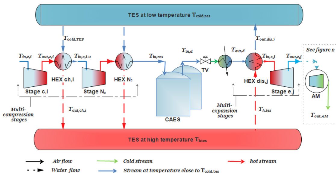
Fig. 1. Schematic diagram of the proposed trigenerative compressed air energy system with the main notations.
