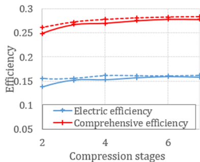
b. T-CAES efficiencies as a function of the number of compression stages.
