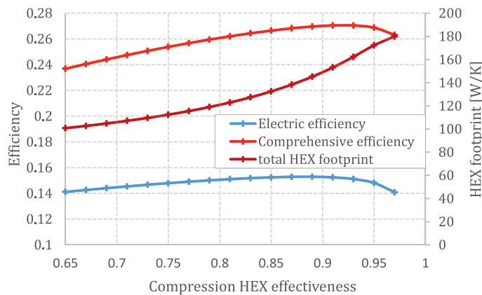
c. T-CAES efficiencies (left axis) and the total HEX footprints (right axis) as a function of the effectiveness of intercooling HEX.
