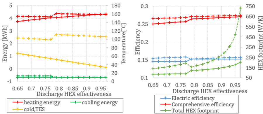
a. Temperature of cold TES (right axis), heating and cooling energy (left axis) as a function of the effectiveness of discharge phase HEX.
