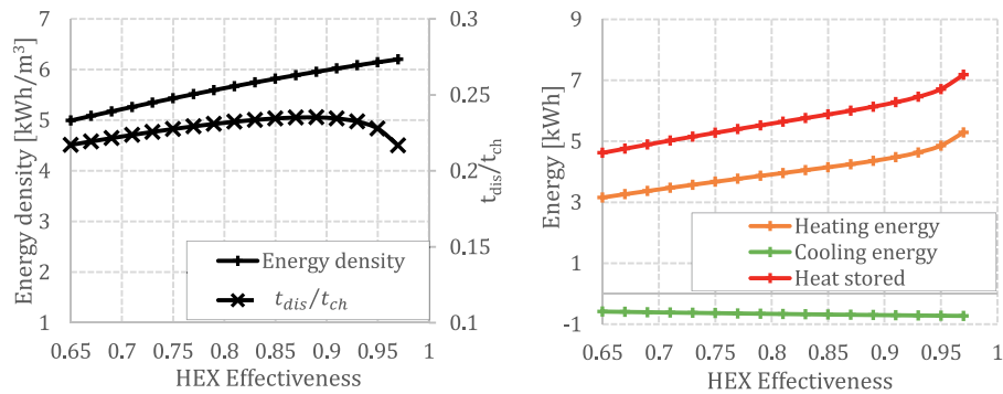
a. Energy density (left axis) and discharge to charge time ratio (right axis) as a function of the effectiveness of intercooling HEX.
