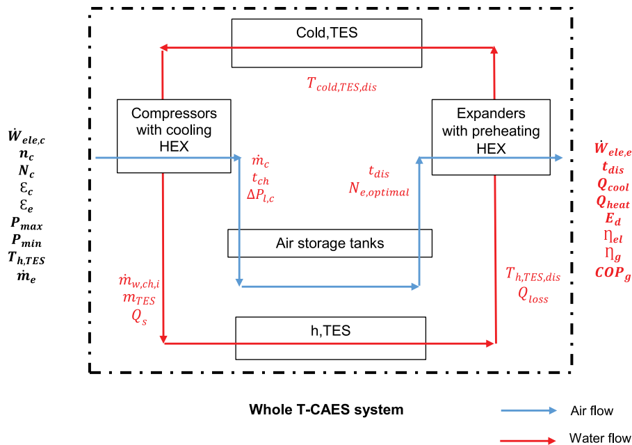
Fig. 4. Block diagram of the thermodynamic model of the whole T-CAES system with main input parameters (black) and output parameters (red). (For interpretation of the references to color in this figure legend, the reader is referred to the web version of this article.)
