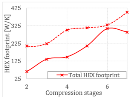
d. The total required HEX footprints as a function of the number of compression stages.
