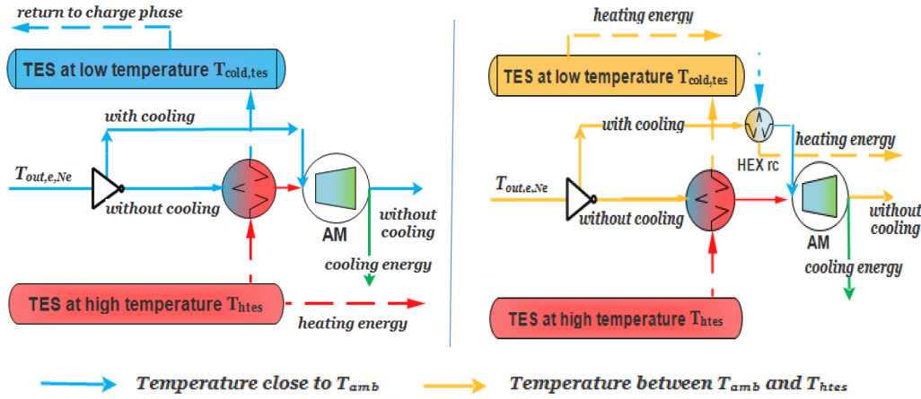
Fig. 2. Schematic diagram of the last expansion stage subsystem (the air motor AM) and temperature levels of streams for the first (left) and the second configuration (right). (For interpretation of the references to color in this figure legend, the reader is referred to the web version of this article.)
