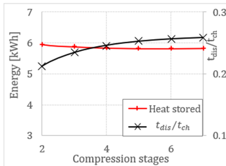
c. Heat stored (left axis) and the discharge to charge time ratio (right axis) as a function of the number of compression stages
