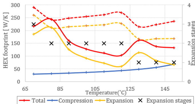
b. Required HEX footprints (left axis) and the number of expansion stages (right axis) as a function of the hot temperature of TES (solid line for first configuration and dashed line for the second).
