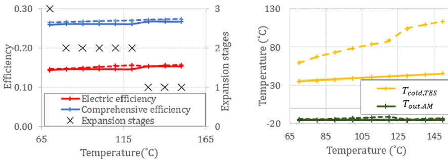
a. T-CAES efficiencies (left axis) and the optimal number of expansion stages (right axis) as a function of the temperature of TES. c. The temperature of AM and of the cold TES as a function of the hot temperature of TES.
