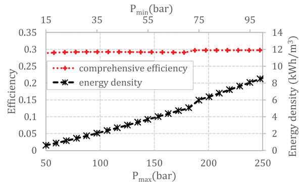
Fig. 10. Comprehensive efficiency (left axis) and energy density (right axis) at constant maximum to minimum pressure ratio as a function of the maximum storage pressure (the variation of the minimum storage pressure is shown in the secondary x-axis on the top).
