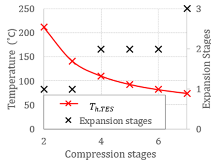
a. Temperature of hot TES (left axis) and required expansions stages (right axis) as a function of the number of compression stages.
