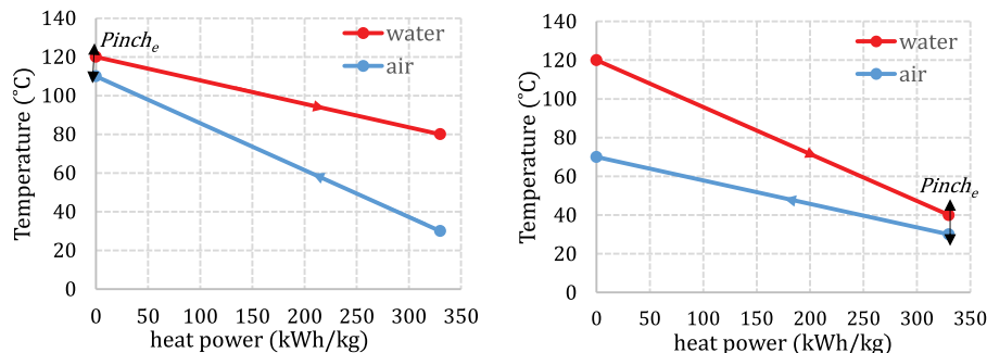
Fig. A1.1. variation of temperature of air and water flow versus heat duty for the first configuration (right) and second configuration (left).
