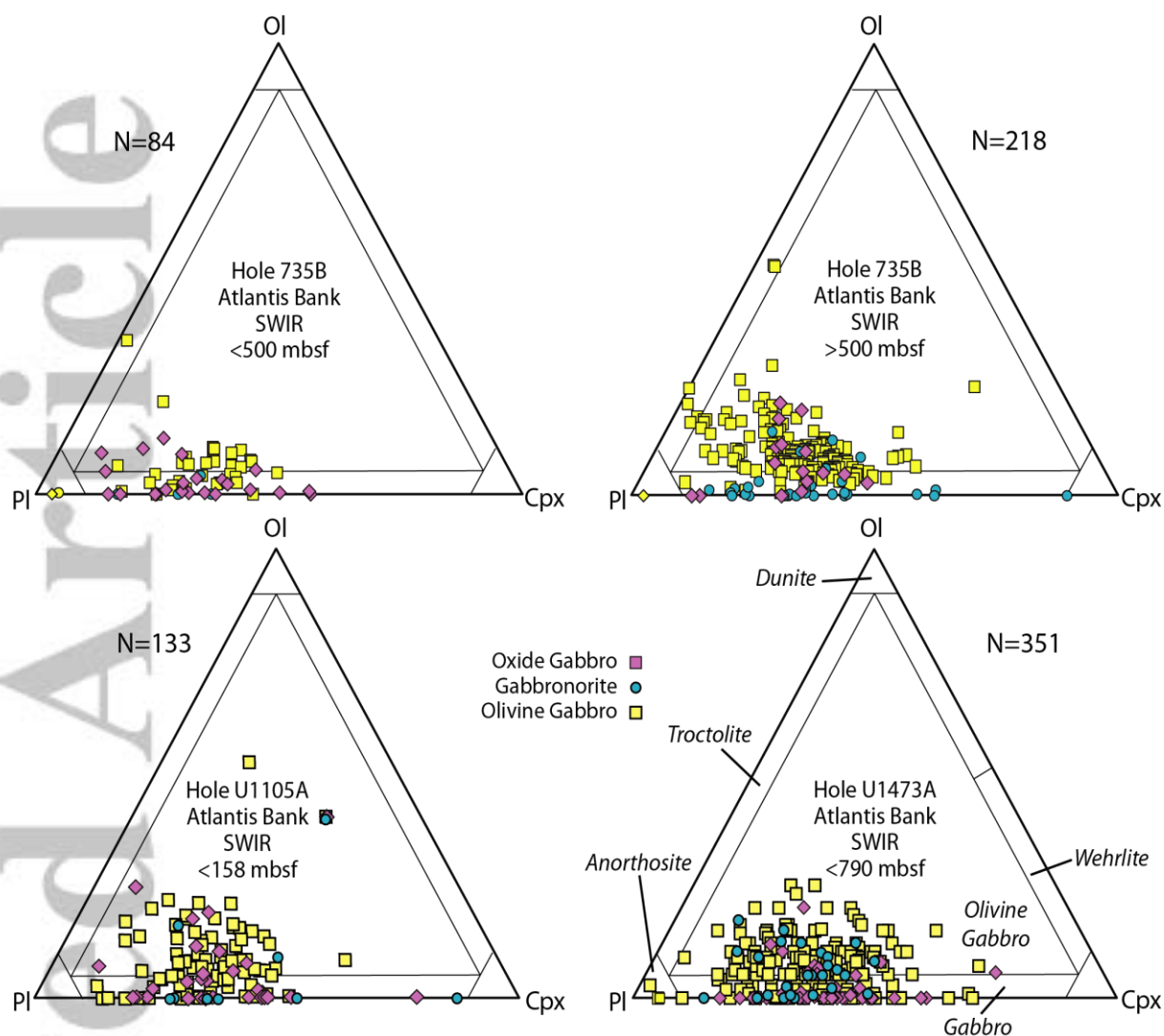
Figure 6. Mineral modes for Atlantis Bank and Atlantis Massif Gabbros: a. Hole 735B 0 to 500 mbsf; b. Hole 735B 500 to 1,508 mbsf; c. Hole 1105A; d. Upper 789.7 m of Hole U1473A (excluding the Expedition 362T section). N equals number of samples point counted.
