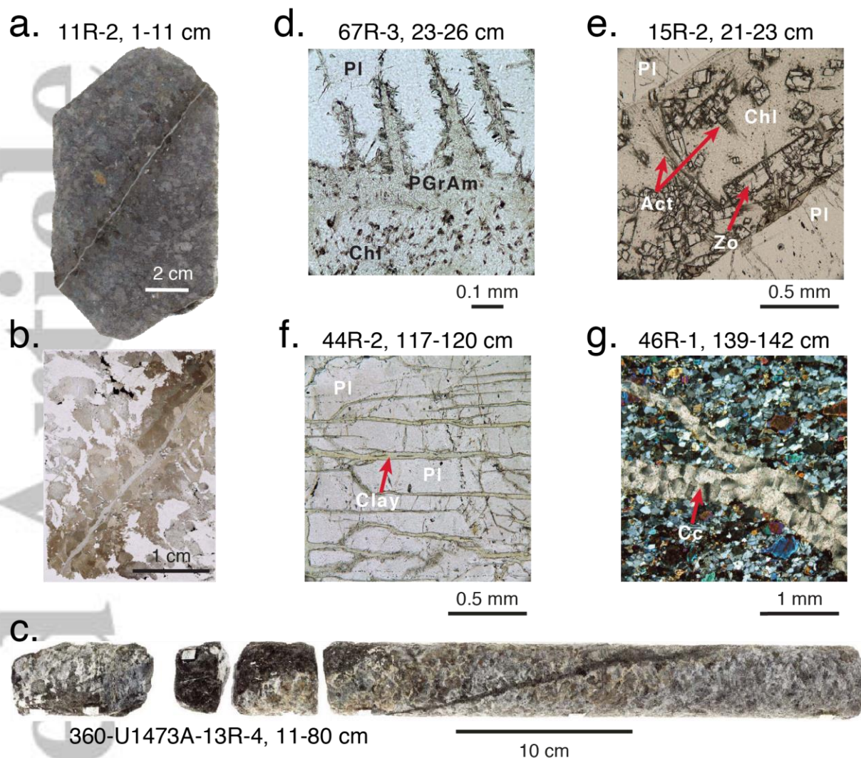
Figure 15. Hole U1473A metamorphic veins: a. Compound amphibole-clinzoisite vein cutting olivine gabbro with alteration corona extending into the fresh olivine gabbro replacing primary Cpx. b. Microphotograph of compound vein in 'A' in plane light consisting of brown and brown-green amphibole sub perpendicular to crystal-plastic foliation, split by a later clinzoisite vein. c. Parallel set of black amphibole veins, one ~5+ mm thick, consisting of mostly of brown and some brown-green amphibole. d. Greenschist facies assemblage in plane light of a felt mass of pale green actinolite and chlorite cutting plagioclase. e. Greenschist facies micro vein crosscutting plagioclase in olivine gabbro consisting of chlorite, zoisite, and actinolite crosscutting plagioclase. f. Yellowish clay microveins crosscutting plagioclase in olivine gabbro. g. Late calcite veins crosscutting a neoblastic domain of plagioclase, Cpx, and olivine in plastically deformed olivine gabbro.
