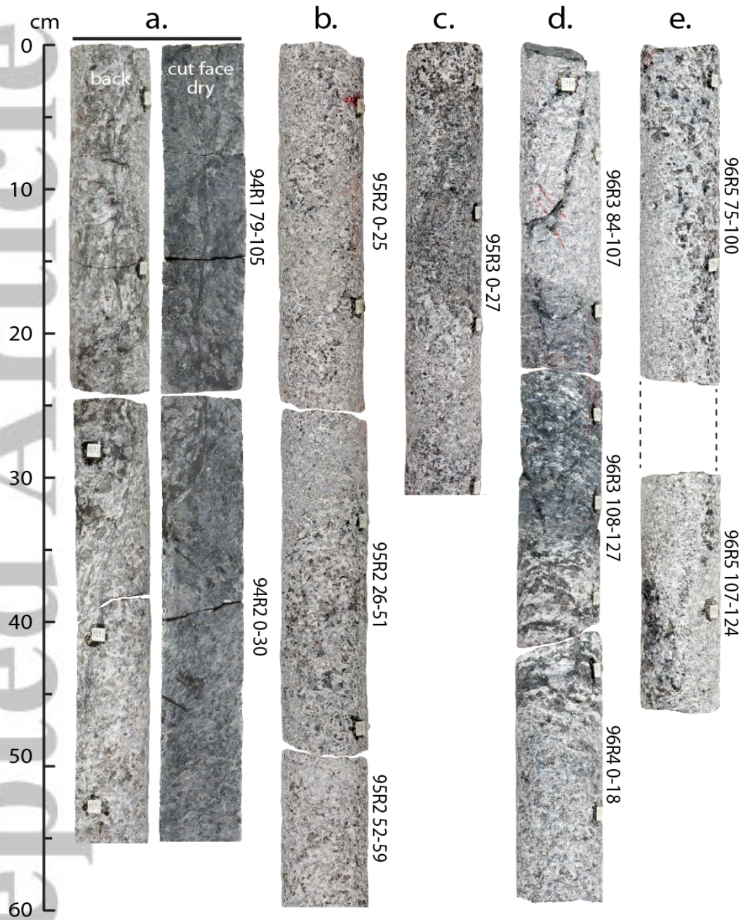
Figure 7. Selected core sections from Expedition 362 T illustrating a variety of different textures and synmagmatic structures found in Hole U1473B. a. Anastomosing oxide impregnated shear zone flanking an anastomosing microgabbro channel cutting up through olivine gabbro. b. Patchy olivine gabbro. c. Augite-rich gabbro patch in patchy textured medium to fine-grained 'isotropic' olivine gabbro. d. Size-graded oxide gabbro ranging from porphyroclastic augen gneiss upward to fine-grained mylonite cutting medium-grained olivine gabbro. e. Anastomosing fine-grained olivine microgabbro channel cutting up through coarse-grained olivine gabbro.
