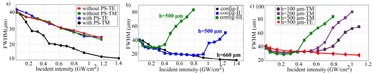
Fig. 4 : a, measured output beam FWHM as a function of input intensity for both TM and TE polarizations without PS and with a PS corresponding to configuration I. b, evolution of output beam width as a function of input intensity for configurations I, II and III for TM polarization. c, evolution of output beam width for configuration III for PS lengths h of 500 \mu\text{m} , 200 \mu\text{m} and 100 \mu\text{m} for TM polarization and for h of 500 \mu\text{m} for TE polarization.
