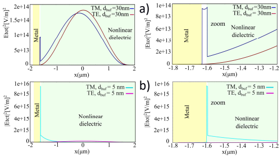
Fig. 2: calculated fundamental TM and TE mode profiles along the X-axis for SiO 2 buffer thickness h equal to 30 nm (a) and 5 nm (b).
