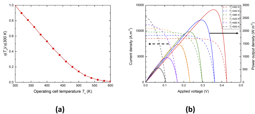
Fig. 2. (a): Loss in efficiency due to thermal losses \eta(T_c)/\eta(300K) as a function of the temperature of the PV device. On the linear part, a temperature coefficient of 0.34 %·K -1 is calculated. (b): J-V and P-V characteristics of the PV cell for different operating cell temperatures T_c . The arrows indicate to which y-axis the curves correspond.
