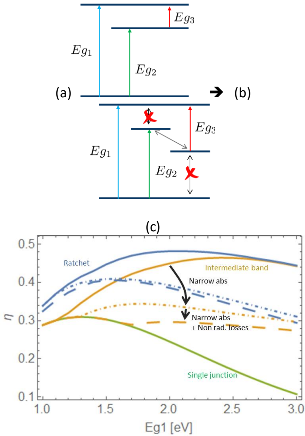
Figure 2 Band diagram of (a) an IBSC and (b) an RBSC with a ratchet implemented in the IB. (c) Efficiencies of the single junction (full green line), IBSC and RBSC, as a function of the largest gap value ( E_{g1} ), in the radiative limit and for an ideal absorption (respectively full orange and blue lines), with a narrow absorption ( \delta E = 250 meV, orange and blue dotted lines), with a narrow absorption and non-radiative recombination ratio of 10^{-3} for the transition E_{g3} (dashed orange and blue lines).
