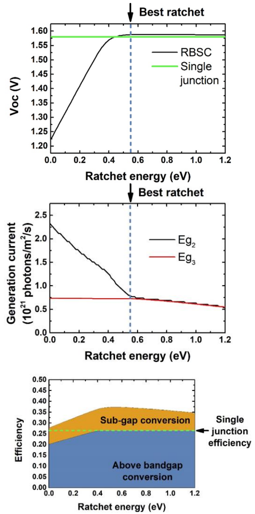
Figure 4 Evolution of recombination, generation and conversion efficiency as a function of the ratchet value, for E_{g1} fixed at 1.86 eV, which is the optimal value for an IBSC when the absorption width is 200 meV and the radiative efficiency 10^{-3} . E_{g2} is optimized for each ratchet value. Top: V_{oc} as a function of ratchet energy \Delta E . The green line represents the value of the single junction for the same E_{g1} . Middle: photogenerated current via transition 2 (middle) and 3 (small gap) as a function of \Delta E . Bottom: fraction converted by the E_{g1} transition and fraction converted with the help of the intermediate band (i.e. converted by E_{g2} and E_{g3} ). The green dashed line represents the efficiency of the single junction with the same E_{g1} .
