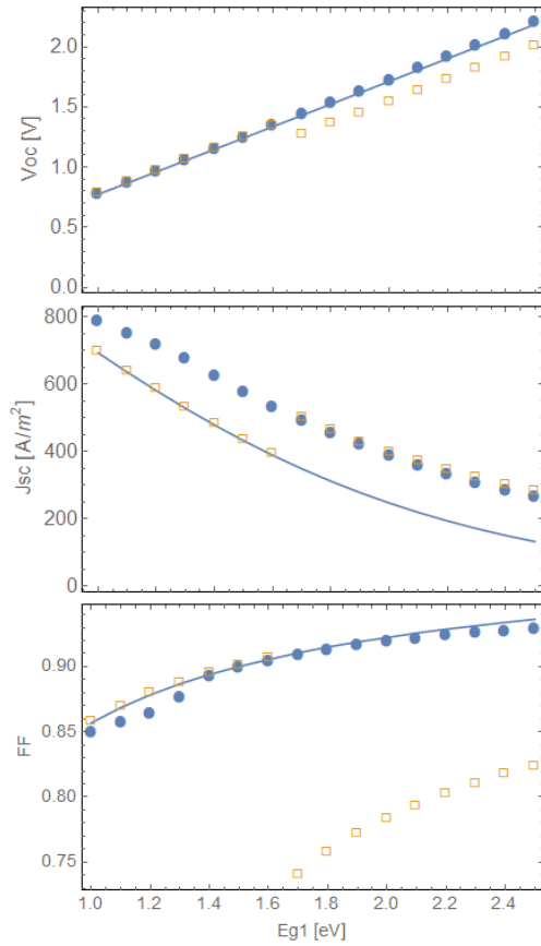
Figure 3 Top: Open-circuit voltage, as a function of the E_{g1} bandgap, for an IBSC with a ratchet (filled blue symbols) and an IBSC w/o ratchet (open yellow symbols). A narrow absorption ( \delta E = 250 meV) and non-radiative recombination ratio of 10-3 are considered for the transition E_{g3} Middle: same for the short circuit current. Bottom: same for the FF.
