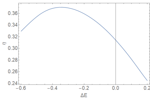
Figure 5 Power conversion efficiency as a function of the ratchet \Delta E in the ideal case with E_{g1} = 2 \text{ eV} and E_{g2} = 1.1 \text{ eV} .
