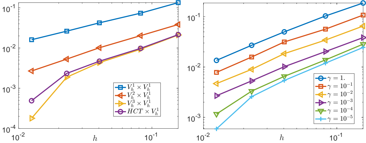
FIGURE 3. (Ex2)- Left : Relative error \|u - u_h\|_{L^2(\mathcal{M})} / \|u\|_{L^2(\mathcal{M})} with respect to h for various approximation spaces (see Table 9); Right : Relative error \|u - u_h\|_{L^2(\mathcal{M})} / \|u\|_{L^2(\mathcal{M})} with respect to h and \gamma for the approximation V_h^2 \times V_h^1 .
