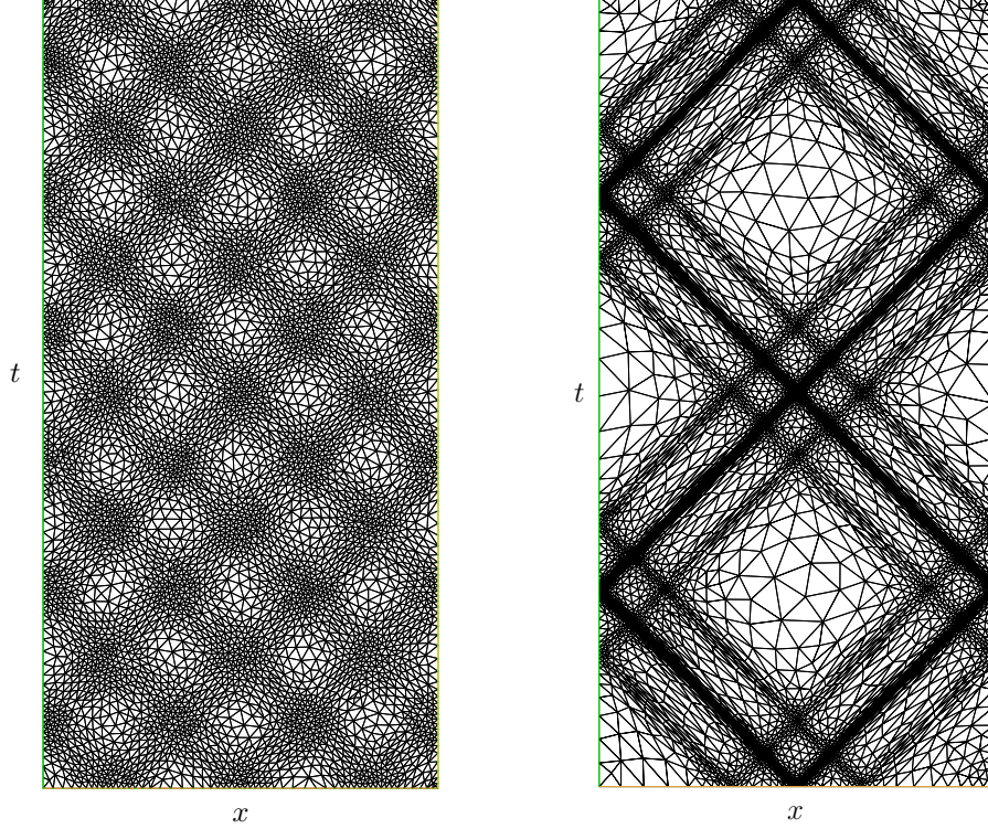
FIGURE 4. Locally refine spacetime meshes for the example 1 ( Left ) and the example 2 ( Right ).
