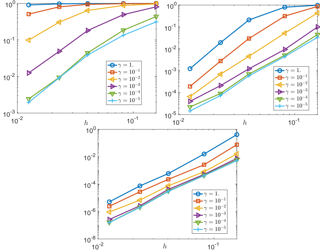
FIGURE 2. (Ex1)- Relative error \|u - u_h\|_{L^2(\mathcal{M})}/\|u\|_{L^2(\mathcal{M})} with respect to h and \gamma for the approximation spaces V_h^1 \times V_h^1 (Left), V_h^2 \times V_h^1 (Right) and V_h^3 \times V_h^1 (Bottom); \gamma^* = 1 .
