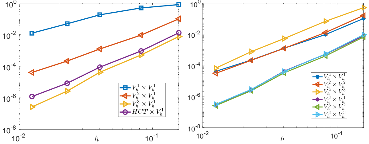
FIGURE 1. (Ex1)- Relative error \|u - u_h\|_{L^2(\mathcal{M})}/\|u\|_{L^2(\mathcal{M})} with respect to h for various approximation spaces (see Table 4); \gamma = 10^{-3} , \gamma^* = 1 .
