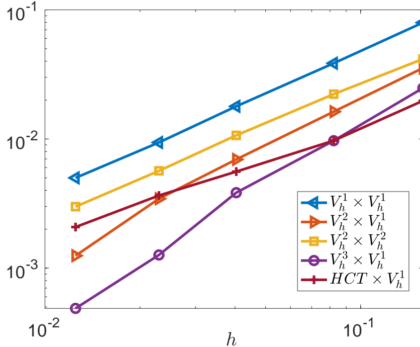
FIGURE 2. (Ex2)- Relative error \|u - u_h\|_{L^2(\mathcal{M})}/\|u\|_{L^2(\mathcal{M})} with respect to h for various approximation spaces (see Table 8).
