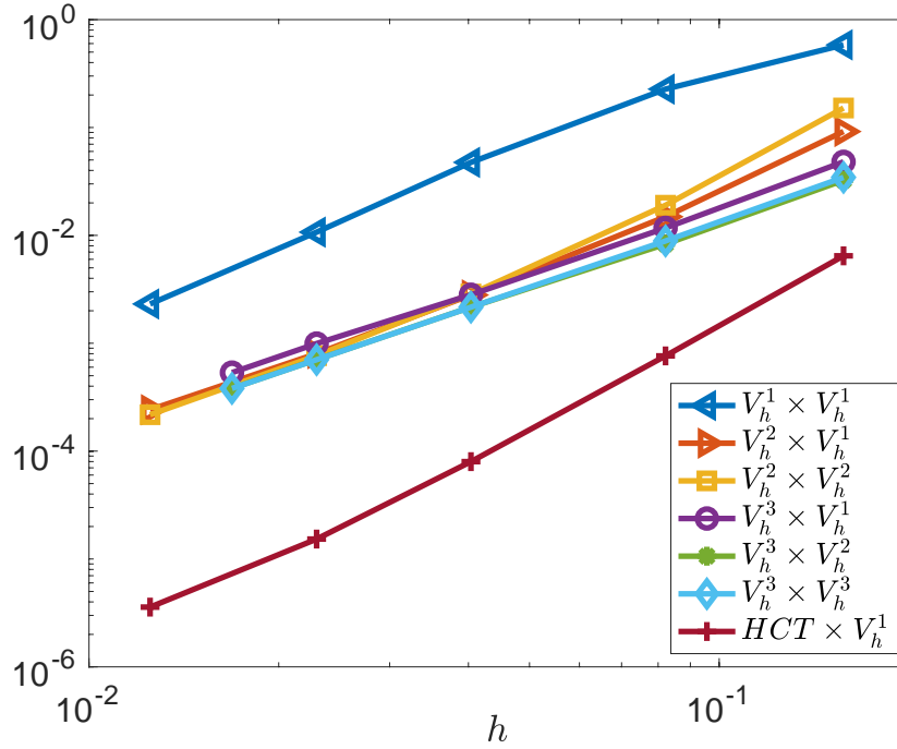
FIGURE 1. (Ex1)- Relative error \|u - u_h\|_{L^2(\mathcal{M})} / \|u\|_{L^2(\mathcal{M})} with respect to h for various approximation spaces (see Table 4).
