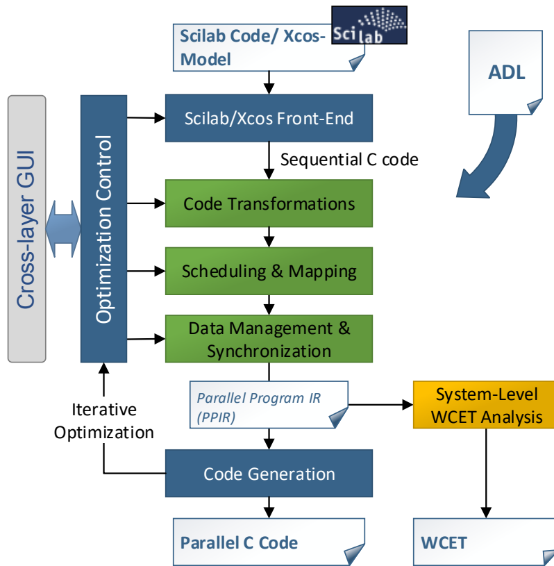
Fig. 4 Structure of the ARGO tool-flow.
