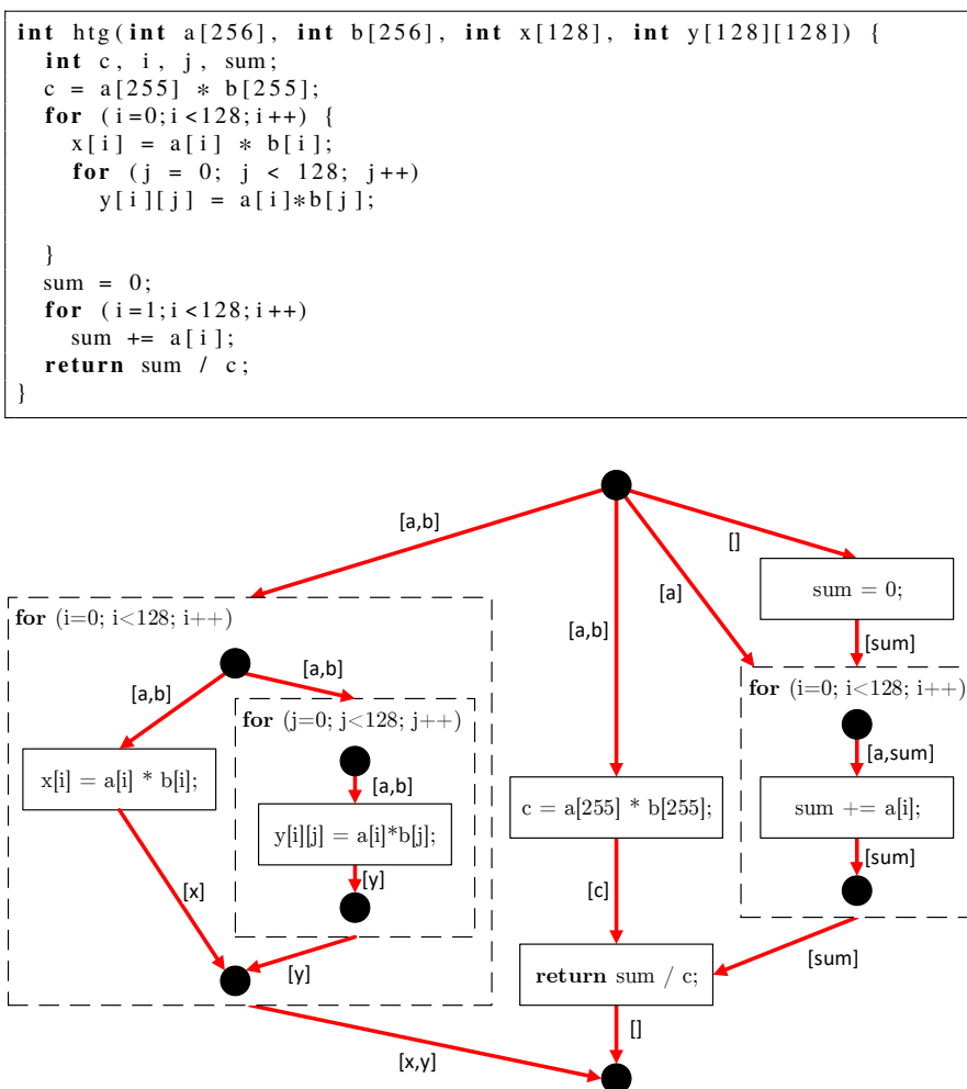
Fig. 5 A source code example and the corresponding HTG with data dependencies for the variables
