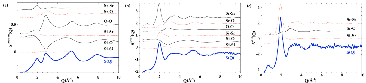
Figure 10: Total structure factors obtained by (a) neutron diffraction, (b) x-ray diffraction and (c) structure factor of first difference determined by anomalous x-ray diffraction at the Sr K-edge for a \text{SrSiO}_3 glass, compared with the weighted partial structure factors determined by RMC modeling.
