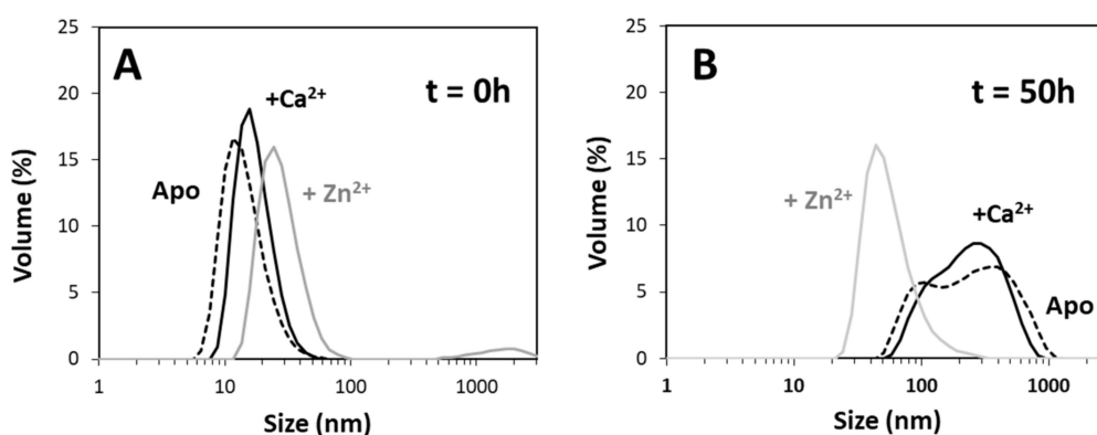
Figure 3. Dynamic light scattering analysis of soluble Tau oligomers. The distribution of particles in solution was analyzed in the beginning of heparin-induced aggregation of 50 \mu\text{M} Tau (A) and after 50 h at the plateau stage (B). Before each measurement samples were centrifuged ( 34,000\times g , 10 min.) and supernatants of the different tested conditions analyzed: apo Tau (dotted line), in the presence of calcium (black line) and in the presence of zinc (grey line). Conditions for the aggregation reaction as those in Figure 1 (see materials and methods for details).
