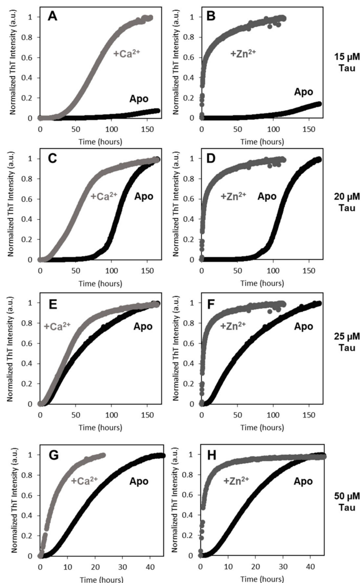
Figure 2. Metal ions promote aggregation of Tau. Tau aggregation in absence (black) or presence of 1.1 mM \text{CaCl}_2 (light gray) or 1.1 mM \text{ZnCl}_2 (dark grey), at increasing hTau441 concentrations: 15 \mu\text{M} (A,B), 20 \mu\text{M} (C,D), 25 \mu\text{M} (E,F) and 50 \mu\text{M} (G,H). All panels are representative of three independent measurements with Tau (at given concentration) at pH 7.4 with 1 mM DTT, 0.5 mg/mL heparin sodium salt, 50 mM NaCl, 1 mM PMSF and 75 \mu\text{M} ThT, under agitation (600 rpm) at 37 °C with or without metal ion. See the experimental section for further details.
