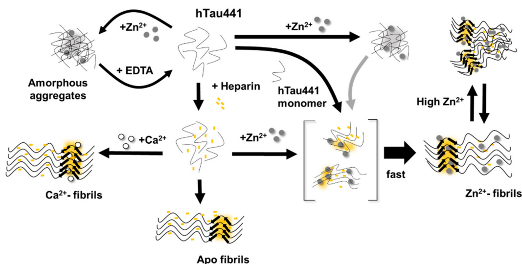
Figure 6. Schematic representation of the multiple conformers generated upon calcium and zinc binding to Tau. The presence of zinc enhances the heparin-dependent aggregation of hTau441 which very rapidly generates a distribution of toxic Thioflavin positive Tau aggregates and fibrils whose formation is also likely promoted by secondary nucleation events involving Tau monomers. Simultaneously, zinc binding to Tau in the absence of an aggregation enhancer promotes the reversible formation of amorphous aggregates, whose formation in the presence of heparin-induced aggregation cannot be excluded nor their involvement as aggregation seeds (grey arrow). It may be speculated that the latter would be favored by high zinc levels which might also promote the formation of amorphous aggregates in ThT-reactive species if low affinity zinc binding is taking place at moieties within the fuzzy coat regions; it is conceivable that these amorphous species are in equilibrium with ordered Zn^{2+} -fibrils. Apo Tau fibrils are formed when hTau441 is incubated in the presence of heparin. See text for details and references.
