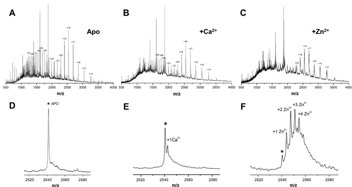
Figure 1. Native mass spectrometry analysis of \text{Ca}^{2+} and \text{Zn}^{2+} binding to hTau441. Native mass spectrum of hTau441 in the apo state (A) and in the presence of calcium (B) and zinc (C), with corresponding details of the +18 charge state multiplet for the apo (D), calcium (E), and zinc (F) bound states. Asterisks (*) denote the peak corresponding to apo (metal-free) hTau441. For assignments see Table S1.
