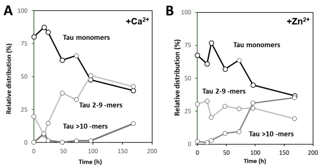
Figure 5. Influence of calcium (A) and zinc (B) on the distribution of Tau oligomers assessed by native mass spectroscopy. The distributions were obtained from peak fitting and deconvolution of the obtained spectra at each time point according to the relative contribution of hTau441 monomers, intermediate oligomers (Tau 2–9 -mers) and large oligomers (> Tau 10-mers).
