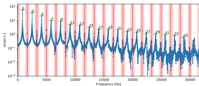
Fig. 2: Frequency spectrum of the impact test (+: identified f_{2n+1} peaks with the corresponding value of 2n+1 ; |: rough antiresonant frequencies f_{2n} ; shaded: discarded peak search zone). Adapted from [23].
