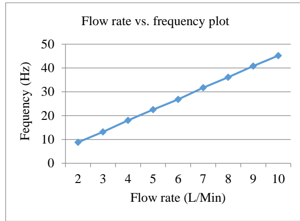
Figure 4: Signal output frequency for different flow rate
