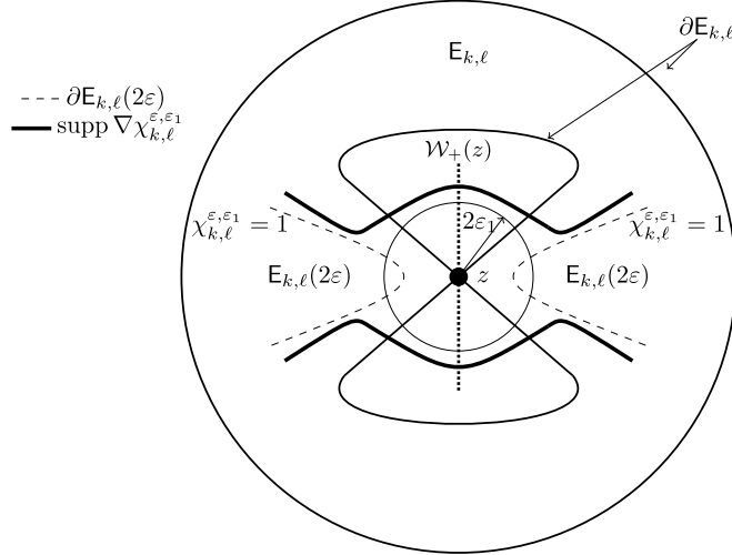
Fig. 6. Schematic representation of the cut-off function \chi_{k,\ell}^{\varepsilon,\varepsilon_1} near z \in (\mathbf{U}_1^\Omega \setminus \mathbf{j}(x_{k,\ell})) \cap \partial E_{k,\ell} . The point z is a saddle point on \partial E_{k,\ell} but is not a separating saddle point as introduced in Definition 13.
