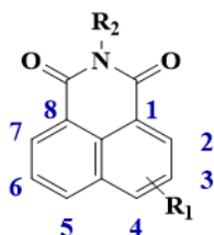
Scheme 1. Chemical structure of 1,8-naphthalimide.
