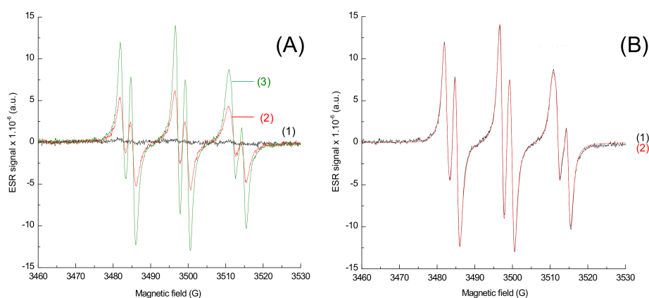
Figure 9. ESR-Spin trapping spectrum of Napht-B1 in combination with \text{Ar}_2\text{I}^+\text{PF}_6^- and 4-dppba in acetonitrile; under air; phenyl- N -tert-butylnitronne (PBN) is used as a spin trap. (A) Experimental spectrum (1) before irradiation; after (2) 40 s and (3) 80 s of irradiation with LED@405 nm ( I \approx 110 \text{ mW}\cdot\text{cm}^{-2} ) exposure; (B) after 80 s of irradiation with LED@405 nm ( I \approx 110 \text{ mW}\cdot\text{cm}^{-2} ) exposure (1) experimental and (2) simulated with the hyperfine coupling constants hfc ( a_{\text{N}} = 14.2 \text{ G} ; a_{\text{H}} = 2.2 \text{ G} ).
