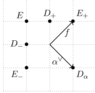
FIGURE 5. Images of divisors in (\mathcal{M} \otimes \mathbb{R})^*
