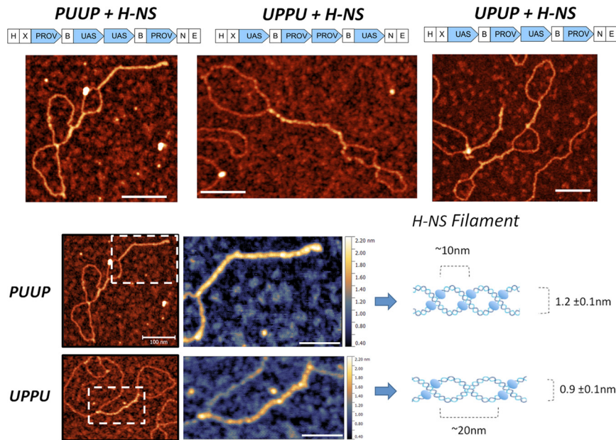
Figure 6. Ultra high vacuum AFM. A , images of different constructs bound by H-NS for H-NS:DNA molar ratio 20:1. Scale bars , 100 nm. B , the close-up view of the PUUP- and UPPU-bridged filaments and the corresponding model with measured shape parameters. The bridging H-NS dimers are indicated by blue ellipsoids . In this model PUUP binds H-NS with high frequency, resulting in higher periodicity of the bridged filament. In contrast, cooperative binding of H-NS to consecutive high-affinity sites of tandem P elements in UPPU stabilizes a plectoneme with high pitch and lower height and periodicity compared with PUUP DNA. We note that the height difference between the PUUP- and UPPU-bridged filaments might be explained by different protein interaction sites involved in H-NS dimer formation (45). Scale bars , 50 nm. H , X , N , B , and E indicate the cleavage sites for HindIII, XbaI, NheI, BamHI, and EcoRI restriction endonucleases, respectively.
