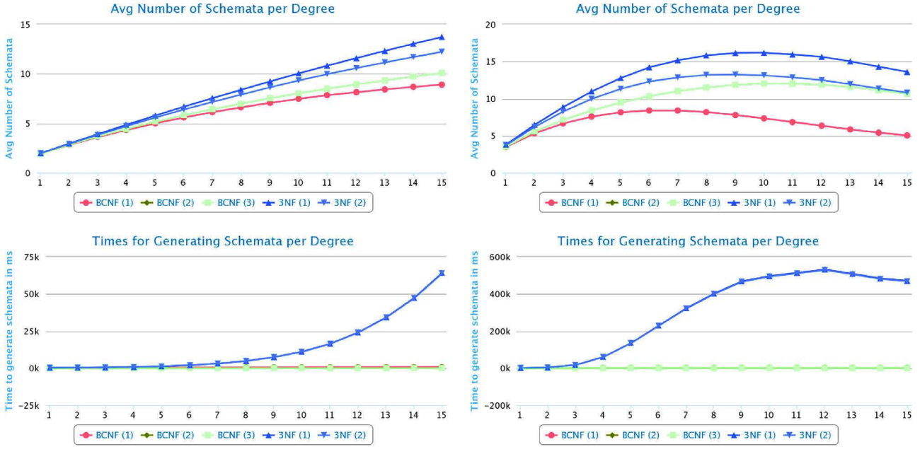
Fig. 8. Average size of decompositions and average times to generate them (y-axis) in the given number k of available c -degrees ( x -axis: k = 1, \dots, 15 ). For a fixed k , the averages were taken over 5000 randomly generated input pFD sets \Sigma over a fixed relation schema with 15 attributes and the number k of available c -degrees. The maximum number s of pFDs in each \Sigma is 15 in the left column and 75 in the right column.
