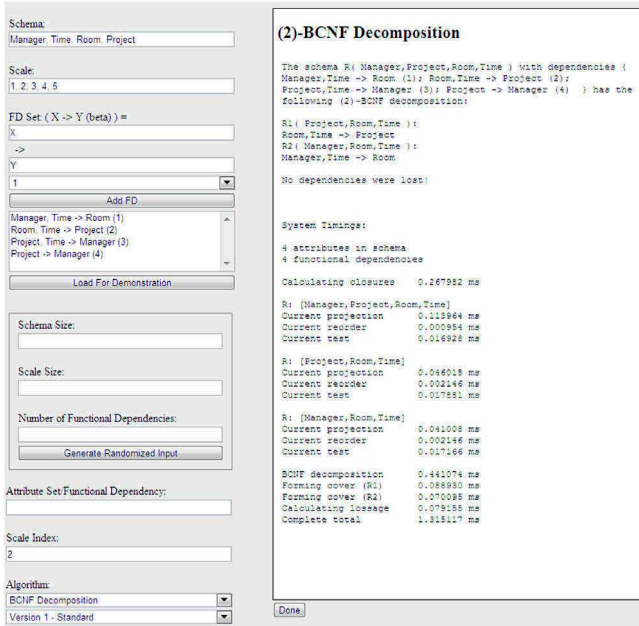
Fig. 7. BCNF example in GUI.
