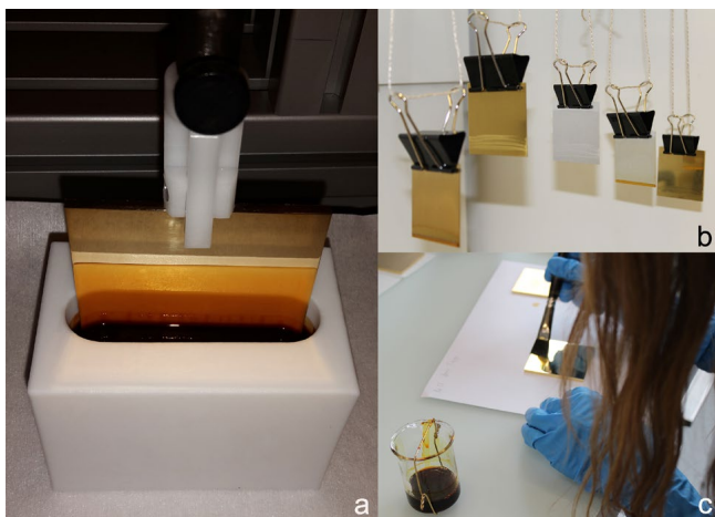
Figure 1. Varnishing of the samples: (a) automated dip coating, (b) manual dip coating and (c) brushing
