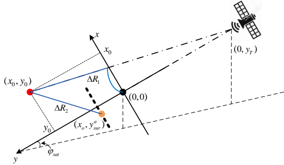
Fig. 4. SAR imaging geometry.
