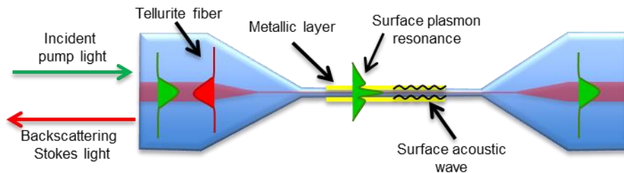
Figure 1: Schematic of the Brillouin backscattering interaction within a tellurite tapered optical fiber coated with gold thin film.
