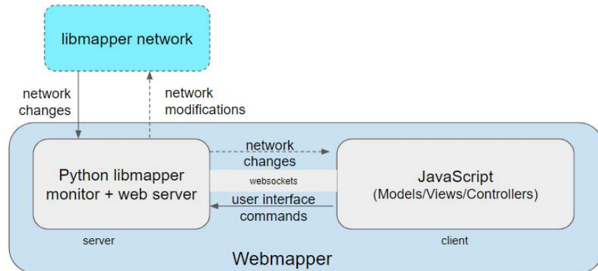
Fig. 1. Webmapper Architecture
