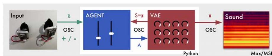
Fig. 4. Schematic representation for the engineering of our instrument.
