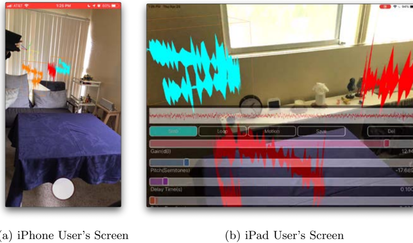
Fig. 2: Multi-user Mode
