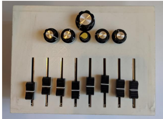
Fig. 3. Image of the interactive device
