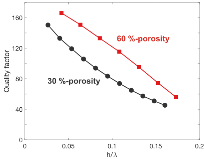
Fig. S5: Evolution of the quality factor at the substrate resonance as a function of the h/\lambda ratio, for two porosity values of 30 % (black circles) and 60 % (red squares).
