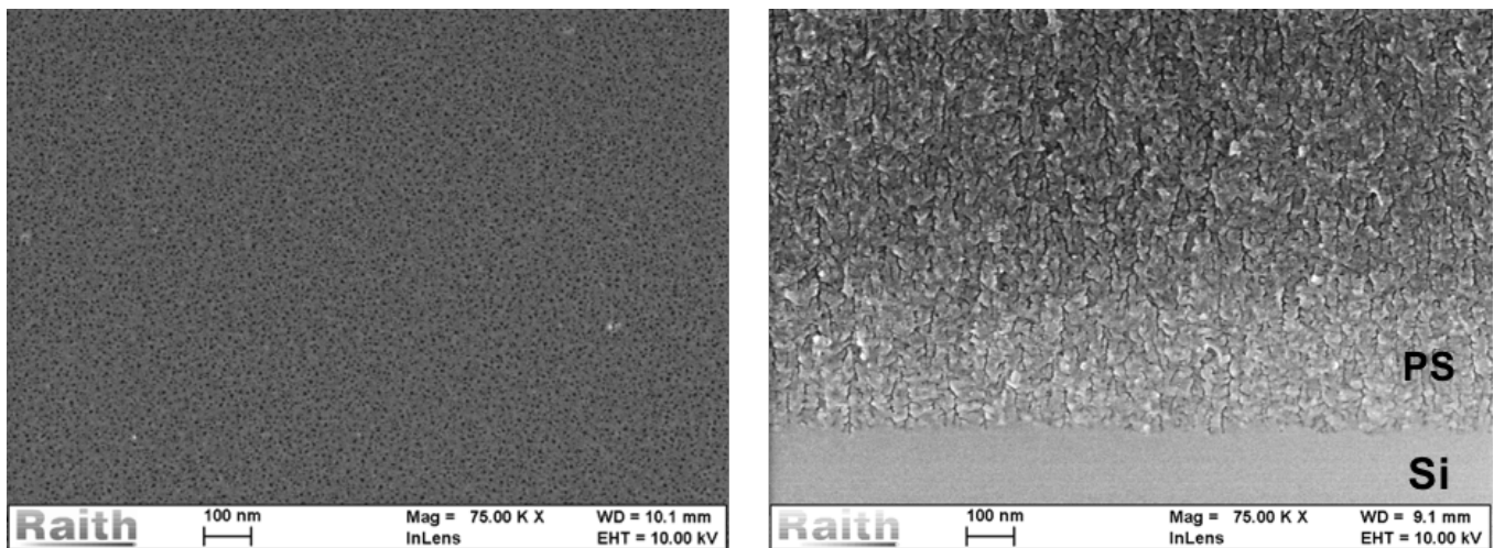
Fig. S1: SEM observations of the porous silicon layer obtained at 50 mA/cm 2 11.5 min, left: top view and right: cross-sectional view.
