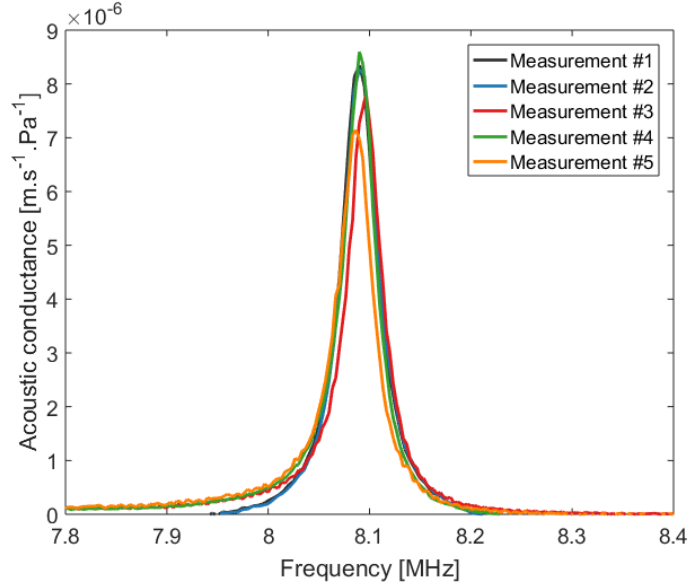
Fig. S3: Acoustic conductances deduced from the measurements of the Si reference plate.
