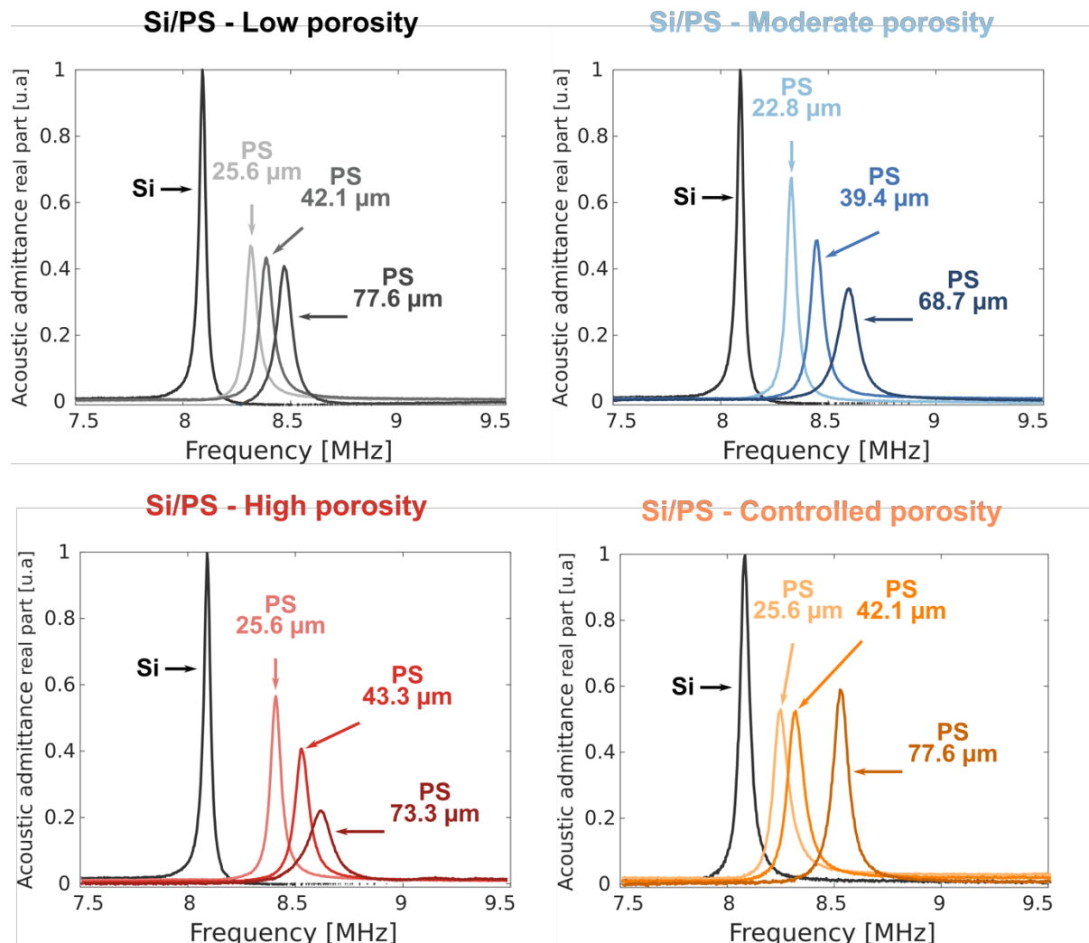
Fig. S4: Normalized real part of the acoustic admittances measured on all the Si/PS samples.
