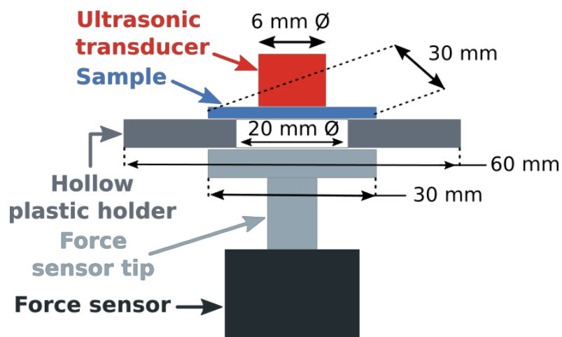
Fig. S2: Schematic representation of the sample setup on the force sensor with the relevant dimensions (unscaled drawing).
