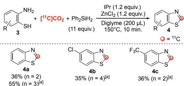
Scheme 2. Cyclizations of aminobenzenethiols with [^{11}\text{C}]\text{CO}_2 . Radiochemical yields are mean values and were estimated from trapped [^{11}\text{C}]\text{CO}_2 within the reactor and are decay-corrected from end of [^{11}\text{C}]\text{CO}_2 trapping inside reactor. [a] diglyme volume = 100 \mu\text{L} .
