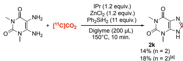
Scheme 3. Intracyclic labelling of theophylline. Radiochemical yields are mean values and were estimated from trapped [^{11}\text{C}]\text{CO}_2 within the reactor and are decay-corrected from end of [^{11}\text{C}]\text{CO}_2 trapping inside reactor. [a] diglyme volume = 100 \mu\text{L} .
