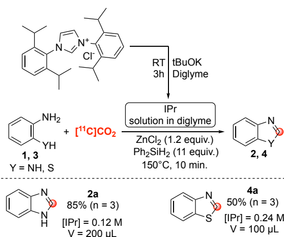
Scheme 4. Cyclization reactions with home-made solution of IPr . Radiochemical yields are mean values and were estimated from trapped [^{11}\text{C}]\text{CO}_2 within the reactor and are decay-corrected from end of [^{11}\text{C}]\text{CO}_2 trapping inside reactor.
