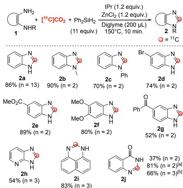
Scheme 1. Cyclizations of aromatic diamines with [^{11}\text{C}]\text{CO}_2 . Radiochemical yields are mean values and were estimated from trapped [^{11}\text{C}]\text{CO}_2 within the reactor and are decay-corrected from end of [^{11}\text{C}]\text{CO}_2 trapping inside reactor. [a] reaction time = 20 min. [b] diglyme volume = 100 \mu\text{L} .
