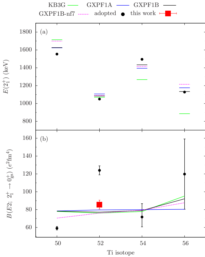
FIG. 12. Comparison of experimental 2_1^+ excitation energies (a) and B(E2; 2_1^+ \rightarrow 0_{\text{gs}}^+) transition strengths (b) with the results of shell-model calculations using the KB3G, GXPF1A, GXPF1B, and GXPF1B-nf7 interactions for ^{50-56}\text{Ti} .
