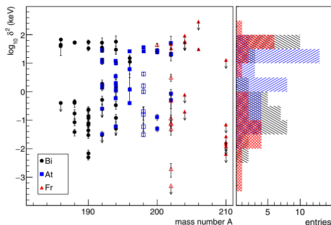
FIG. 11. Representation of the reduced widths for odd-odd At, Bi, and Fr nuclei in the region N < 126 . Open symbols indicate the values deduced from this work, solid symbols represent literature values [4,5,11,28–30,32–34]. In most cases, each isomer has only one unhindered decay ( 10 \lesssim \delta_\alpha^2 \lesssim 100 ), while the other \alpha -decay lines are hindered by at least a factor of 100.
