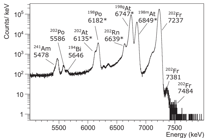
FIG. 2. Relevant part of the \alpha -sum spectrum as recorded by the silicon detectors Si1 and Si2 at mass A = 202 . Energies are given in keV and the lines used for energy calibration are marked with an asterisk (*) and taken from the literature [11,20,21]. The \alpha line at 5478 keV is from ^{241}\text{Am} calibration sources, mounted on the wheel of the windmill.
