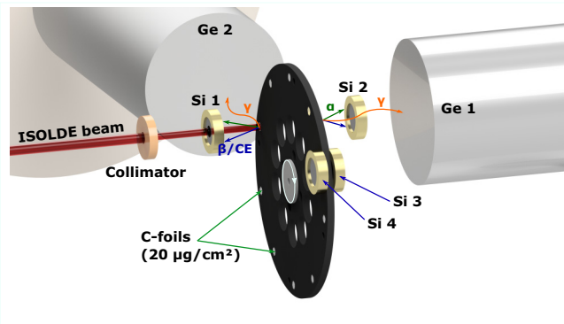
FIG. 1. A schematic view of the windmill detection setup. A radioactive beam from ISOLDE was implanted in one of ten carbon foils of \sim 20 \mu\text{g}/\text{cm}^2 thickness, mounted on a rotatable wheel. Four silicon detectors were employed for the detection of electrons, \alpha and fission particles. Two germanium detectors were placed outside the vacuum chamber for \gamma -ray detection. Illustration from Ref. [18].
