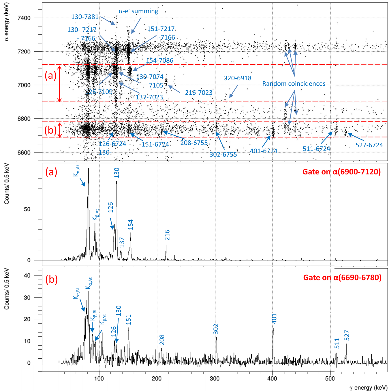
FIG. 3. The top panel depicts part of the prompt \alpha - \gamma coincidences, relevant for the decay of ^{202}\text{Fr} , observed between the detectors Si1 and Si2 at the implantation position and the germanium detector Ge1. The width of the time gate was set to 600 ns. The identified \alpha - \gamma groups are denoted with their respective energies in keV. Panels (a) and (b) show the random-subtracted \gamma -energy spectra coincident with the ranges of \alpha -decay energies indicated by the broken red dotted lines on the upper plot. The energies of the \gamma lines are given in keV.
