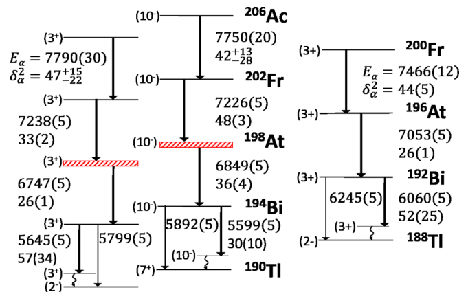
FIG. 10. Schematic view of the main \alpha -decay chains of the ground and isomeric states of ^{206}\text{Ac} up to ^{190}\text{Tl} (left) and for ^{200}\text{Fr} - ^{188}\text{Tl} (right). The \alpha -decay energies and reduced widths are given in keV and taken from the literature [4,11,13,28] or from this work (for ^{200}\text{Fr} decay). The excitation energy of the isomer in ^{198}\text{At} (cf. red hatched lines) has been used as the reference to calculate the excitation energies of parent and daughter nuclei in Table VIII.
