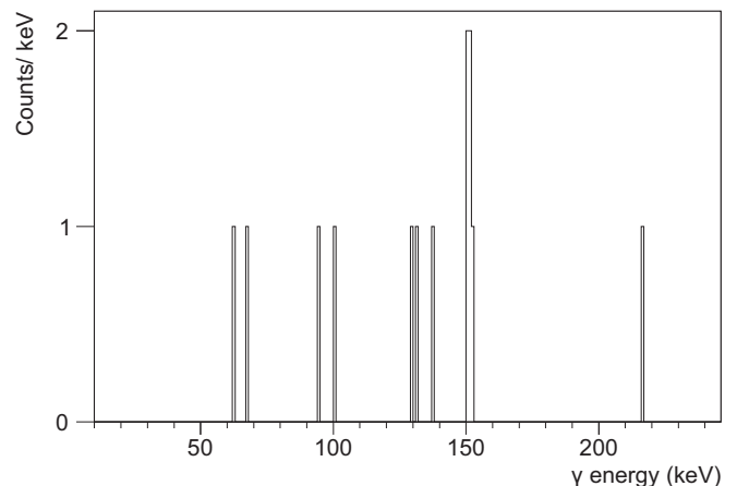
FIG. 4. \gamma -energy spectrum in prompt coincidence with pairs of coincident \alpha(7217) - \gamma(130) .
