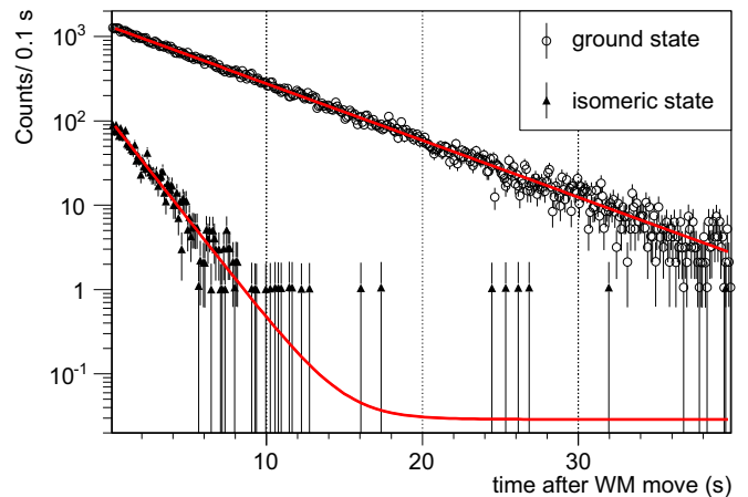
FIG. 6. Timing distributions of \alpha particles, recorded by detectors Si3 and Si4, with respect to the movement of the windmill (WM). The data are corrected for dead-time effects, which were monitored by a 10 Hz pulser (see Ref. [17]). The closed triangles and open circles correspond to the \alpha -decay lines of ^{198}\text{At} at 6753 keV (isomeric state) and 6854 keV (ground state). Fits to the data are shown by the red lines, yielding half-life values of 4.47(10) and 1.28(10) s for the ground and isomeric level, respectively.
