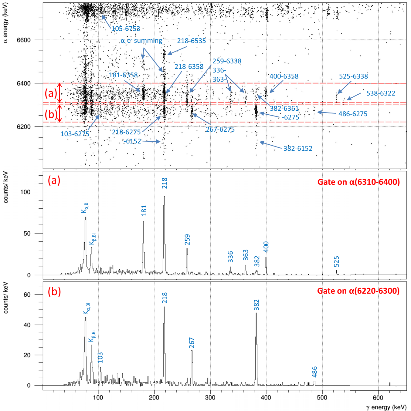
FIG. 7. Similar to Fig. 3, but the range of the \alpha - \gamma plot (top) and projections (a) and (b) are now relevant for the ^{198}\text{At} - ^{194}\text{Bi} decay.
