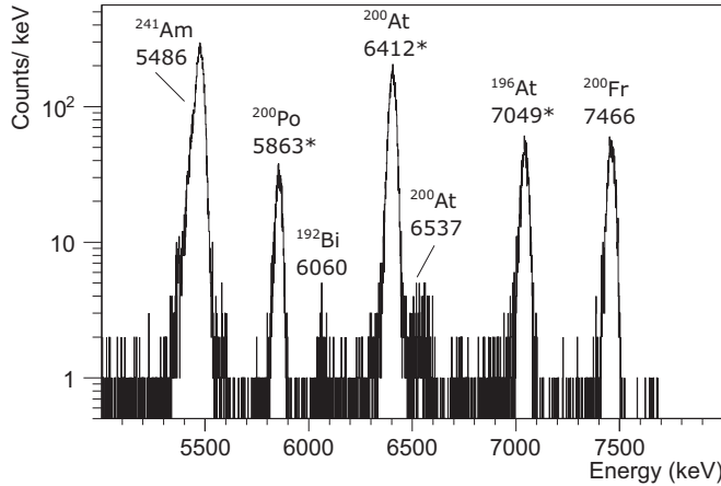
FIG. 8. Relevant part of the singles \alpha spectrum as recorded by the silicon detectors Si1 and Si2 at the implantation station at mass 200. Energies are given in keV and the lines used for energy calibration, taken from the literature [25,26], are marked with an asterisk (*). The \alpha line at 5.486 MeV is from ^{241}\text{Am} calibration sources, mounted in the wheel of the detection system.
