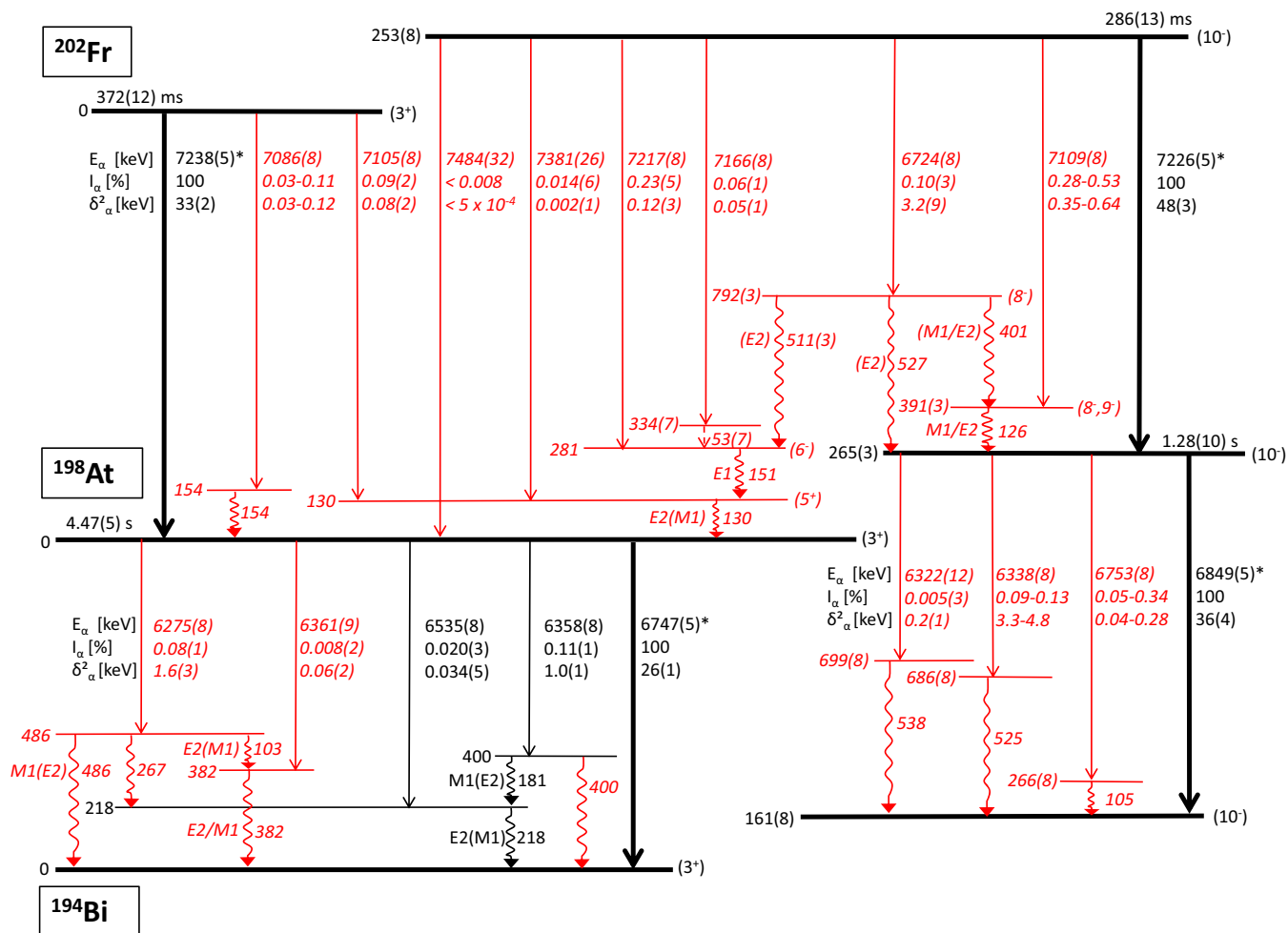
FIG. 5. The \alpha -decay scheme of ^{202}\text{Fr} and its daughter ^{198}\text{At} as deduced from this work. All energies are given in keV. The yet-unobserved transition of 53(7) keV following the \alpha decay of ^{202}\text{Fr} is indicated by a dashed arrow. The lifetimes of ^{202g,m}\text{Fr} are taken from Ref. [11]. The main \alpha lines in the ^{198}\text{At} decay, marked with an asterisk (*), have been used for the energy calibration of the silicon detectors. Therefore, their energies are taken from the literature [11]. New transitions and levels are indicated in red, with the corresponding information written in italics.
