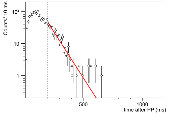
FIG. 9. Timing behavior of \alpha particles with energies between 7350 and 7550 keV, attributed to the decay of ^{200}\text{Fr} , with respect to the arrival of a proton pulse (PP) on the ISOLDE target. Implantation is stopped after 200 ms, as indicated by the dotted line. The data are fit with a simple exponential curve without background, shown by the red line, yielding a half-life of 52(3) ms for ^{200}\text{Fr} .
