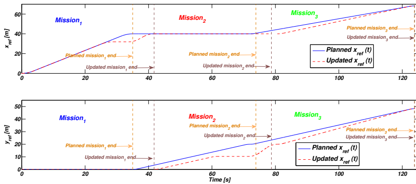
Fig. 8. Planned and updated reference position trajectories
