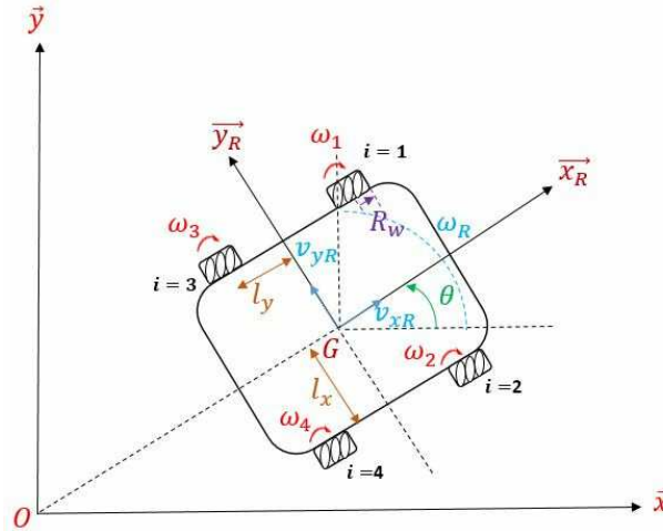
Fig. 2. Geometry of a 4-mecanum wheeled robot.
