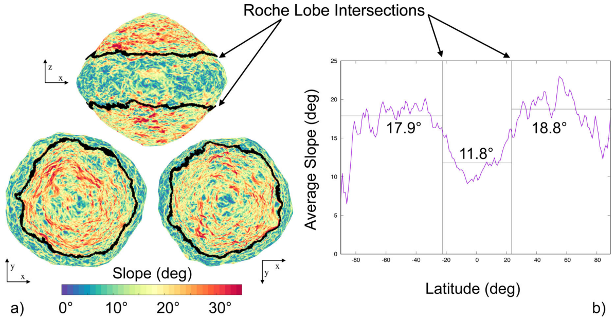
Figure 3: Surface slope distributions on Bennu in relation to the rotational Roche lobe. a , Slope distribution for a 3-m-resolution shape model of Bennu shown with the rotational Roche lobe intersection with the surface, marked with the thick black line. The slope transition is seen to closely follow the lobe intersection region. b , Longitudinally averaged slope as a function of latitude, showing the average slopes within and outside of the lobe. The averaging is over 1-degree-latitude bins, and thus at the average lobe transition latitude will capture some regions on the other side of the lobe. If the averaging is performed exclusively within the lobe the average slope decreases to 11.7°, and the overall average slope outside of the lobe is 18.4°.
