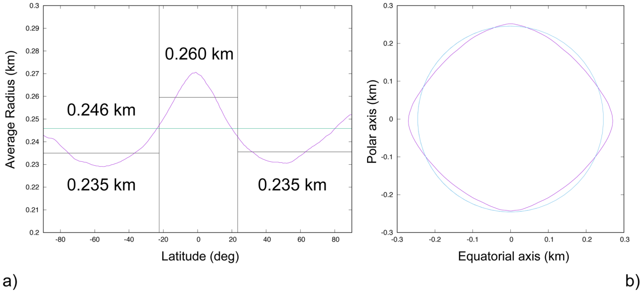
Figure 5: The averaged Benu shape shows global characteristics associated with a landslide failure. a , The longitudinally averaged Benu radius as a function of latitude, shown in purple. The green line is the globally averaged radius and the black lines are the averages inside and outside of the lobe. b , Benu’s shape profile (purple line) compared with its average radius (blue). The smaller radius at mid-latitudes, pole radii close to the mean radius, and exuded equator constitute a predicted profile for a global surface landslide [19].
