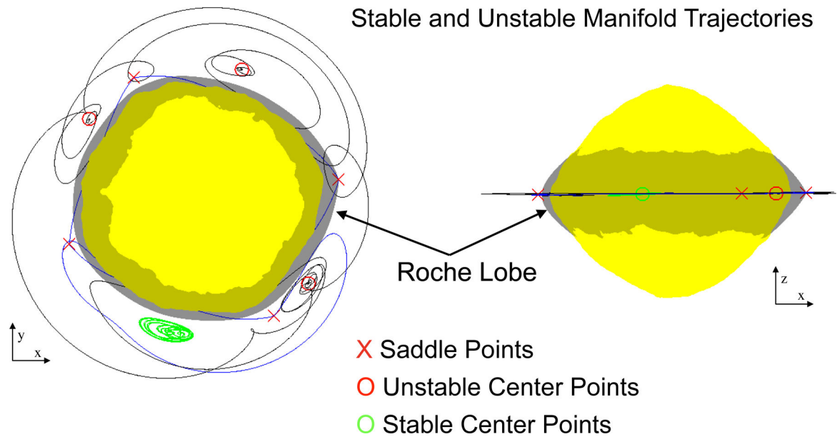
Figure 2: Equilibrium points in the Bennu-fixed frame, shown with stable and unstable manifolds emanating from the unstable points, and showing a stable trajectory in the vicinity of the stable equilibrium point.
