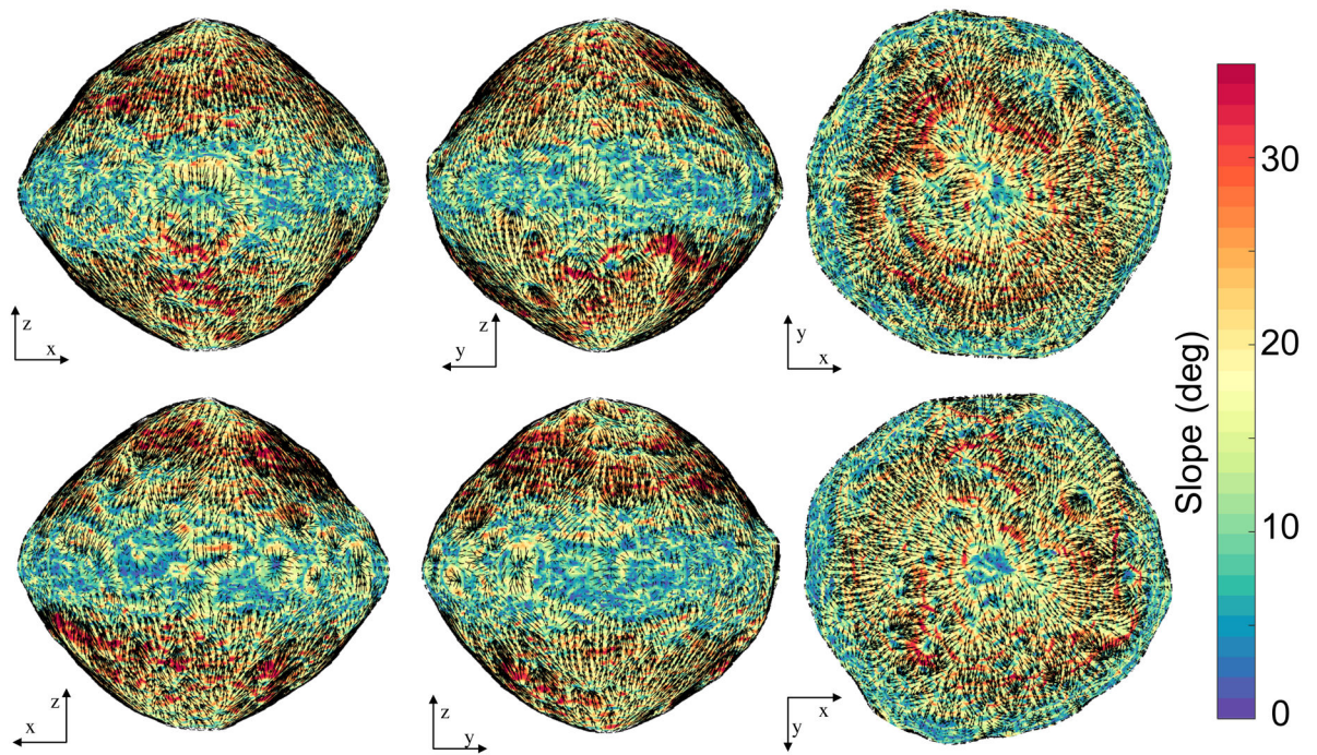
Figure 1: Global map of slope distributions across Bennu.
