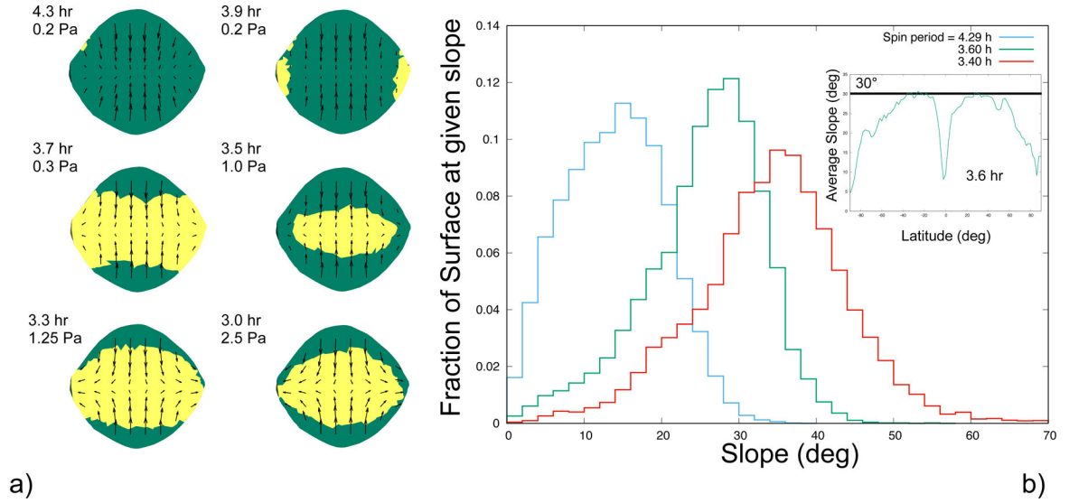
Figure 4: Failure patterns as a function of Bennu spin rates.
