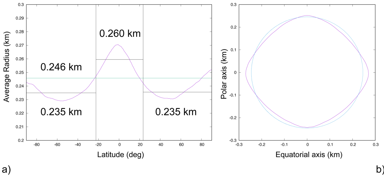
Figure 5: The averaged Bennu shape shows global characteristics associated with a landslide failure.
