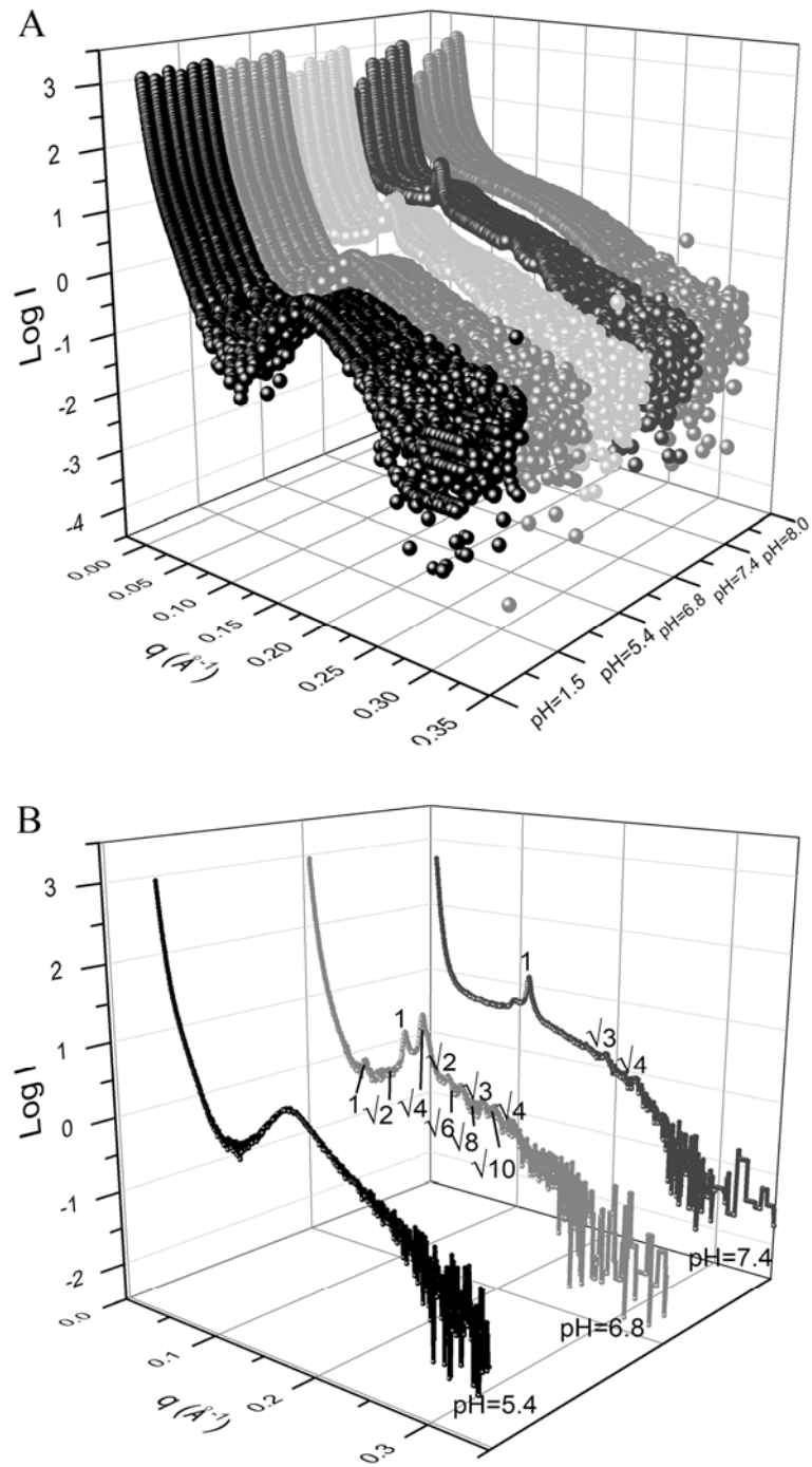
Figure 1. (A) SAXS patterns of pH-sensitive lyotropic liquid crystalline nanocarriers as a function of the pH values of the aqueous environment. Six compositions (MO-OA, MO-0.9OA-0.1BJO, MO-0.8OA-0.2BJO, MO-0.7OA-0.3BJO, MO-0.6OA-0.4BJO and MO-0.5OA-0.5BJO) (in the order from front to back) are presented for each pH value: pH=1.5, pH=5.4, pH=6.8, pH=7.4 and pH=8.0. (B) Indexing of the Bragg peaks of the inverted hexagonal (H II ) (pH 7.4) and the inverted cubic (pH 6.8) liquid crystalline phases for the BJO-containing nanocarriers MO-0.9OA-0.1BJO is shown together with the pattern recorded at pH 5.4 and corresponding to a sponge phase or an emulsified microemulsion (EME).
