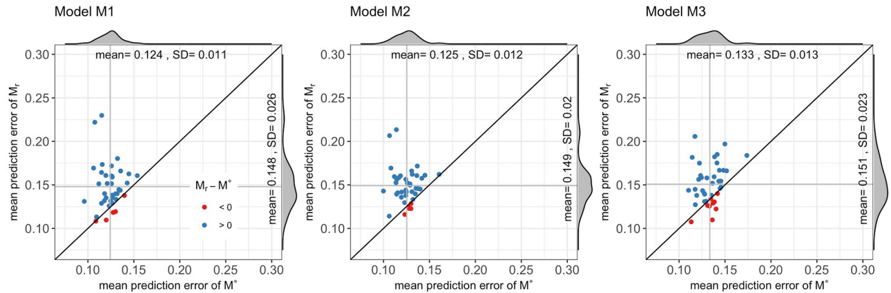
Fig 7. Mean predictive errors. The MPEs of model M^* are smaller than the MPEs of models M_r , in the majority of the cases (blue dots). Furthermore, in the cases where the MPEs of models M^* are bigger (red dots), the differences are small (close to identity line).
