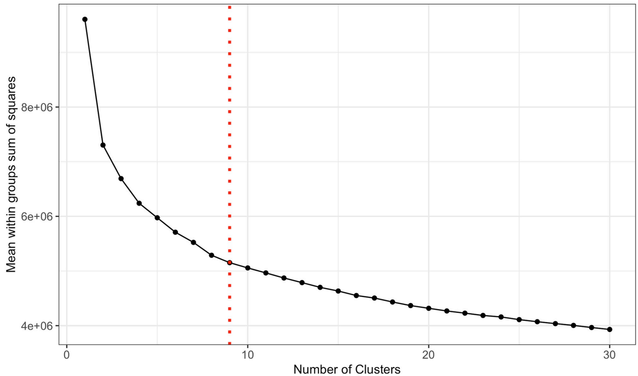
Fig 3. Determining the number of clusters k . The sum of squared errors for k -means clustering of the 624,490 OD-routes with k = 1, . . . , 30. After k = 9 the decrease in the mean WCSS is marginal.
