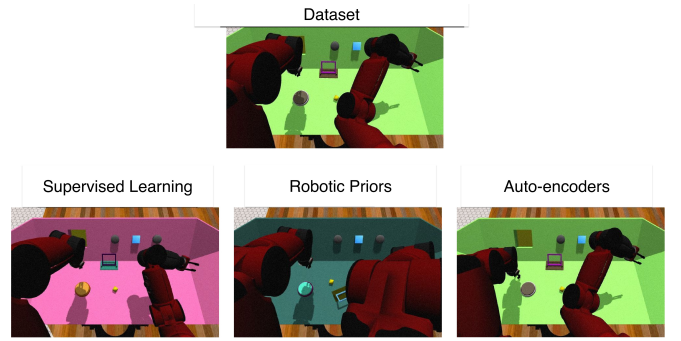
Fig. 7. Nearest neighbors retrieved for each of the models on the Colorful75 Dataset 4. The neighbors should represent the same button-hand relative position. Performance is shown in a left-right decreasing performance for the supervised (hand position) learning, 5 robotic priors and the autoencoder (better seen in video material). We can see that Supervised learning and Robotic Priors are very close (in terms of hand position), whereas the autoencoder matches the color of the table but misses the hand position (its representation doesn't encode the relevant information)
