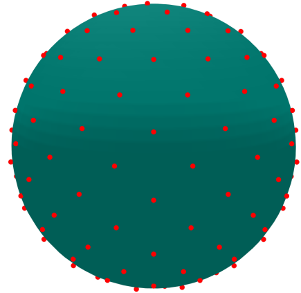
Fig. 1. Uniform sampling of the sphere.
