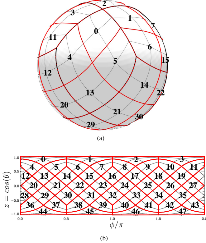
Fig. 4. Proposed scanning order for the case when S-blocks are 2 \times 2 and sphere is pixelized into 192 pixels. S-blocks are processed ring by ring starting from the north pole. Red lines are the border of the S-blocks and black thin lines are the border of the pixels. (a) S-blocks on the sphere. (b) Cylindrical projection of S-blocks and pixels.
