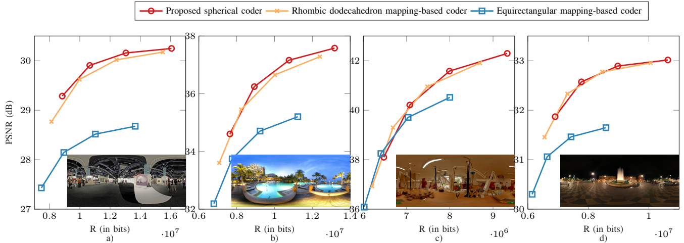
Fig. 5. RD curves of 4 images for different coding methods. (a) Image Exhibition. (b) Image Pool. (c) Image workshop. (d) Image Plaza.
