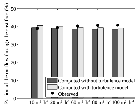
Figure 2. Distribution of outflows between the downstream faces in the observations and for different model characteristics.
