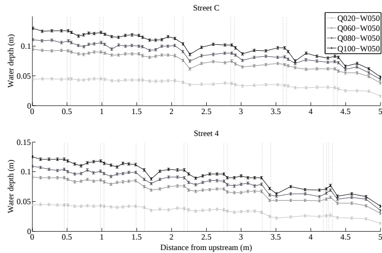
Figure 4. Observed water depths in streets C and 4 for inflow discharges varying between 20 and 100 \text{ m}^3 \text{ s}^{-1} . Dashed vertical lines indicate the intersections.
