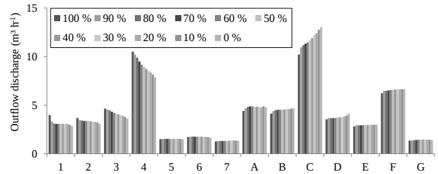
Figure 13. Observed outflow discharges in each street for when the inflow through the west face ( \phi_{\text{west}} ) is varied between 100 and 0 %.
