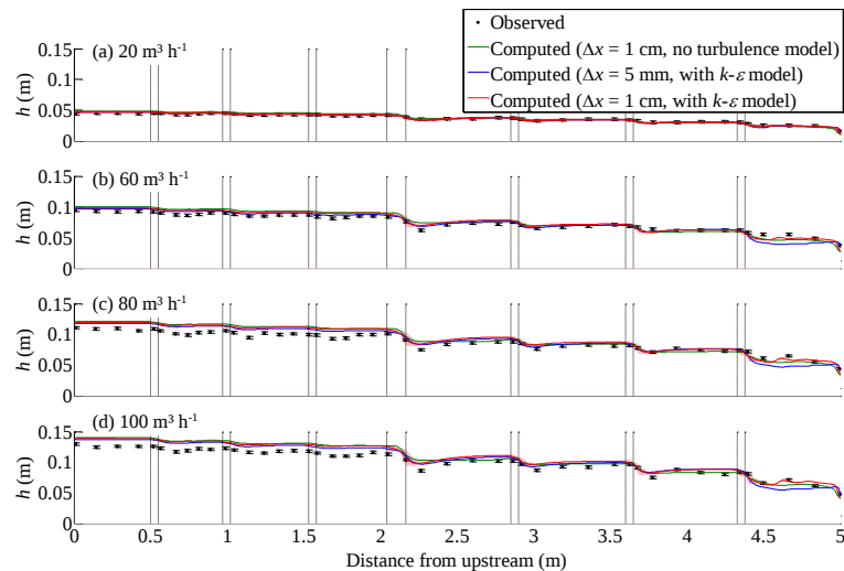
Figure 5. Observed and computed water depths h for inflow discharges varying between 20 and 100 \text{ m}^3 \text{ h}^{-1} in street C. The shaded area (■) represents the range of variation in the crosswise direction of the computed water depths ( \Delta x = 1 \text{ cm} , with k-\varepsilon model).
