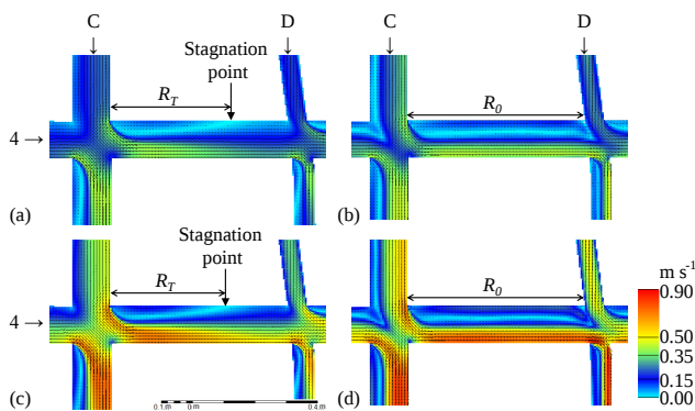
Figure 10. Velocity fields computed with (a, c) and without (b, d) the turbulence model for tests Q020-W050 (a, b) and Q100-W050 (c, d). Grid size: 5 mm.
