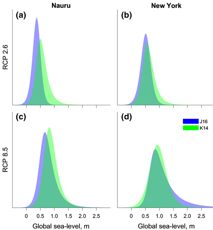
Fig. 2 Probability density functions for sea level in Nauru (Pacific island) and New York in 2100 for RCP2.6 and RCP8.5. Green colour corresponds to the results from Kopp et al. (2014), named as K14, and blue to the results from Jackson and Jevrejeva (2016), J16
