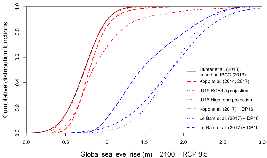
Fig. 3 Projections of globally mean sea level rise (GMSL, in m) by 2100 under RCP8.5 represented in a cumulative distribution diagram. (Church et al. 2013a; Kopp et al. 2014; Jackson and Jevrejeva, 2016; Kopp et al. 2017; Le Bars et al. 2017). Here, the curve labelled as “Hunter et al. (2013), based on IPCC (Church et al. 2013a)”, is a modification of the median and likely range provided by Church et al. (2013a), following the interpretation of Hunter et al. (2013), which assumes a symmetric Gaussian extrapolation of the IPCC likely range and median values. DP16 is reference to the estimate of contribution from Antarctica ice sheet by DeConto and Pollard (2016), which is used in studies by Kopp et al. (2017) and Le Bars, et al. (2017); JJ16 is reference to Jackson and Jevrejeva, 2016 (including RCP8.5 scenarios, labelled as JJ16 RCP8.5 projection, and the high-end scenario, labelled as JJ16 High-end projection)
