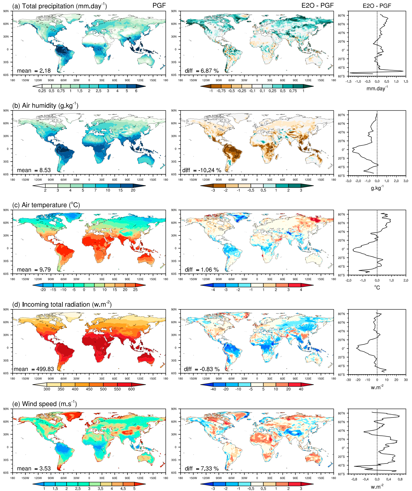
Figure 3. Global distributions of the annual means of NCEP-GPCC-based PGF meteorological data (left panels) and their differences with ERA/Interim-MSWEP-based E20 atmospheric forcing variables (center panels). Zonal averages of these differences are also shown in right panels.
