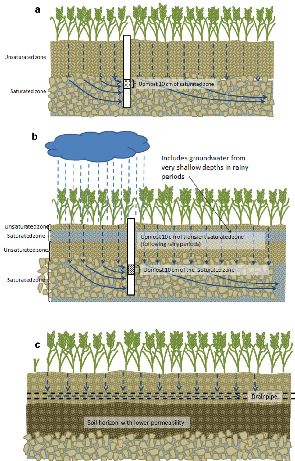
Fig. 2 Definition of relevant groundwater under option 1 (includes a ) single zone of saturation, b transient zone of saturation, and c tile drain water saturation). In all 3 settings, the water table can vary throughout the year. In setting b , the transient saturated zone may actually be the result of a rise in the water table, with no unsaturated zone between the lower and upper saturated zones
