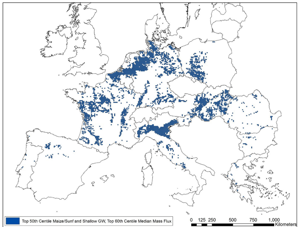
Fig. 16 Example of a mass flux map for an herbicide calculated with GeoPEARL for the usage area in the EU (i.e., country with registration and crop of interest)
