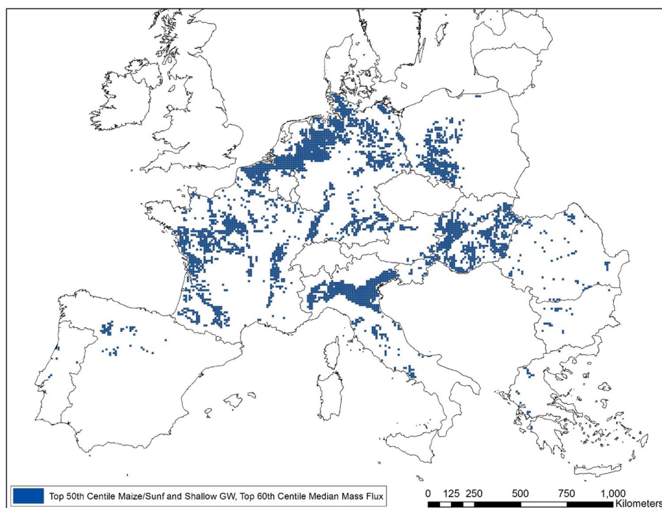
Fig. 16 Example of a mass flux map for an herbicide calculated with GeoPEARL for the usage area in the EU (i.e., country with registration and crop of interest)
