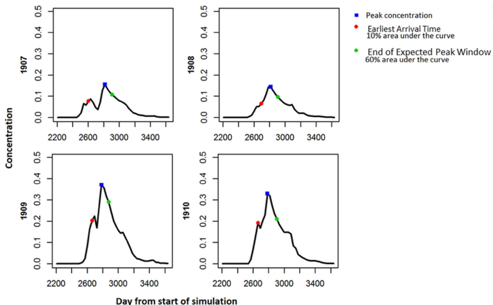
Fig. 37 An example of an active ingredient which has a multi-peak concentration time-series. The use of the PEC max as an estimate of pesticide arrival at the target depth would be inaccurate
