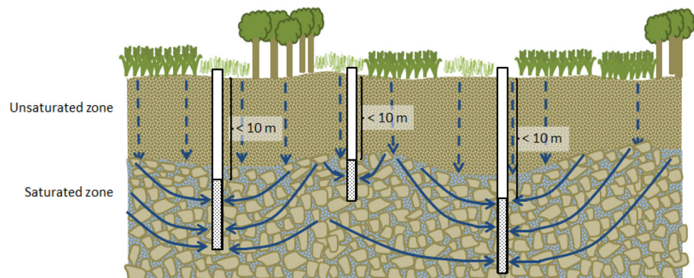
Fig. 6 Definition of relevant groundwater under option 6. Option 7 is the same as option 6 except that samples collected from drinking-water pumping stations where the apparent age of the water is greater than 50 years are not considered vulnerable enough to be included in determining whether option 7 is being met
