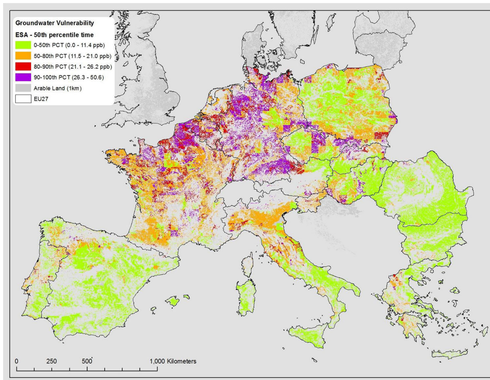
Fig. 12 Example of a vulnerability map for an herbicide calculated with GeoPEARL for usage in the EU. The vulnerability is depicted in percentiles of the range of leaching concentrations (50th percentile in time for each simulation) calculated by the model
