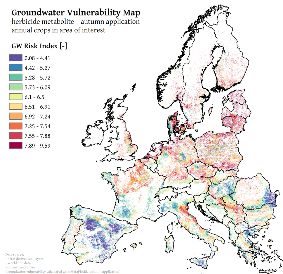
Fig. 13 Example of a vulnerability map calculated with MetaPEARL for the annual cropping area in the EU. The vulnerability is depicted in terms of the HAIR groundwater risk indicator derived from the leaching concentrations calculated by the model
