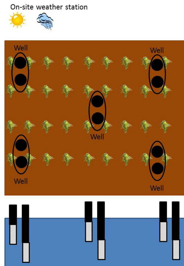
Fig. 7 Schematic diagram of an in-field groundwater monitoring study
