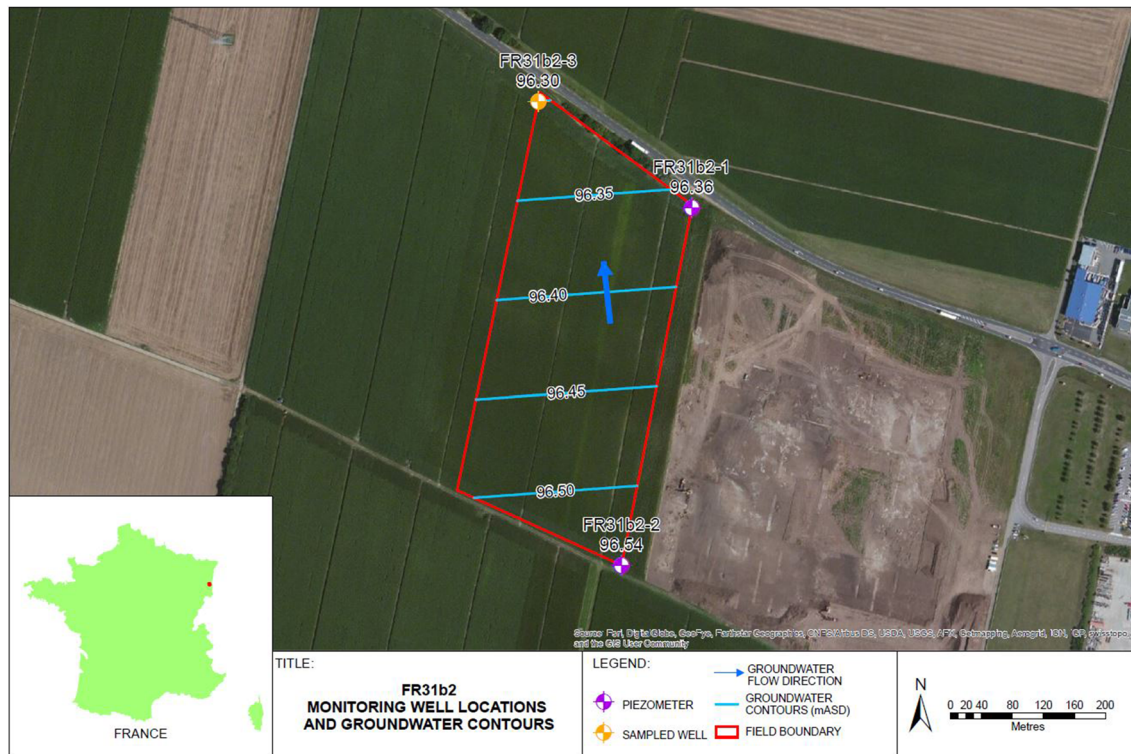
Fig. 25 Example edge-of-field layout with three wells at one site for triangulation to determine the down-hydraulic gradient sampling well
