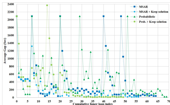
FIGURE 6 Convergence patterns of the inner loops with initialization methods for Saturation (S) scenario on Lyon6V network. [default is All-or-nothing initialization]
