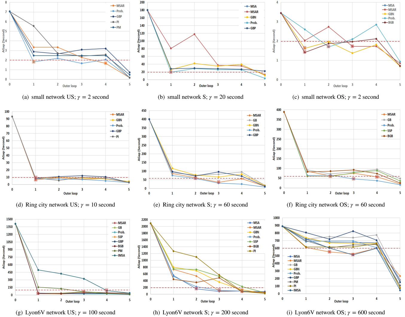
FIGURE 5 Convergence patterns for the swapping algorithms of all scenarios. There are 3 different saturation levels per each network: Under Saturation (US), Saturation (S) and Over Saturation (OS). \gamma denotes the satisfaction threshold.
