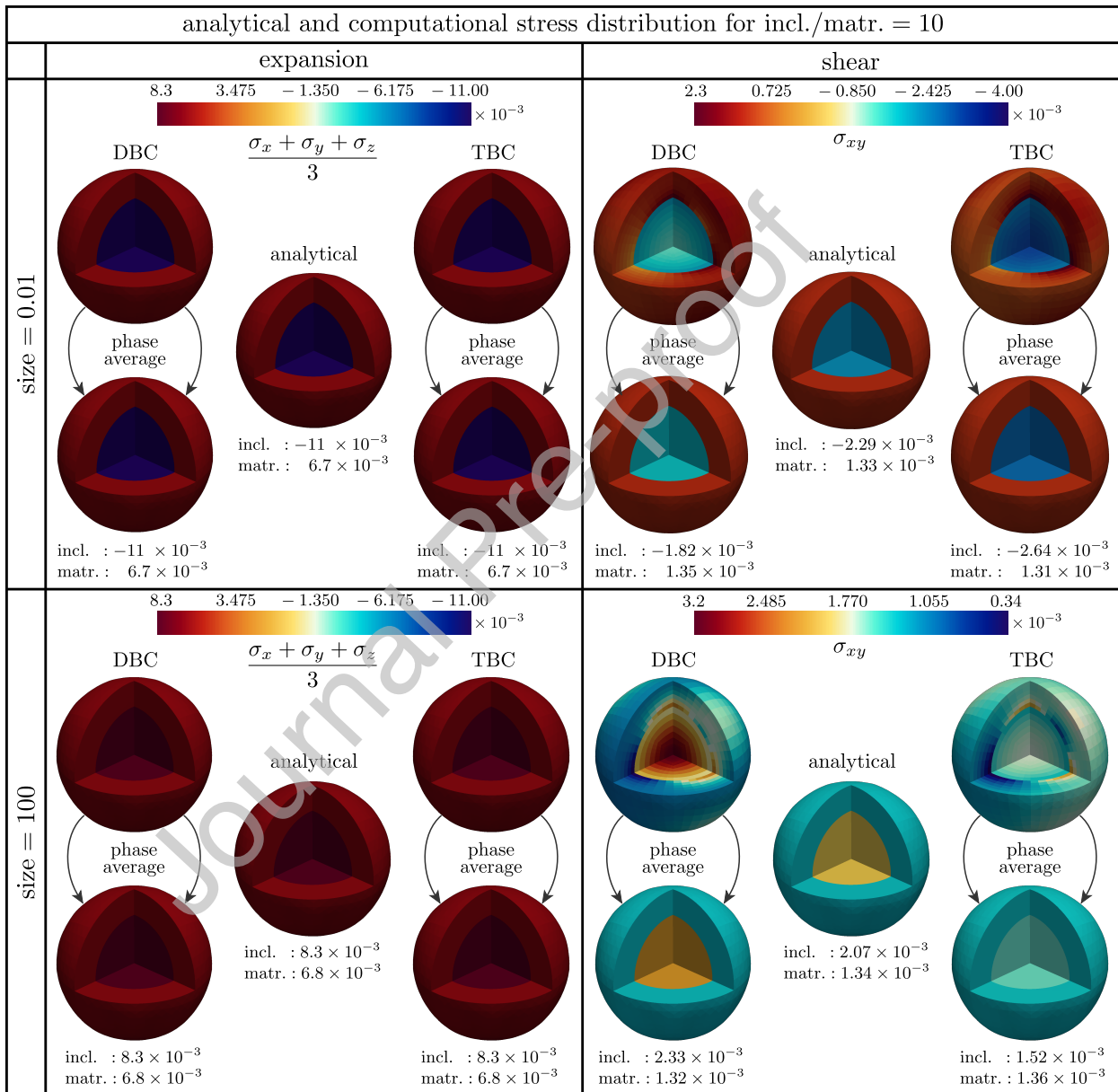
Figure 14: Comparison of the analytical and numerical stress distributions within the RVE at different sizes for \text{incl./matr.} = 10 . On each block, the top micro-structures correspond to the local stress distribution due to DBC and TBC. The analytical stress distribution is shown at the center. The bottom micro-structures render the average of the computational stresses due to DBC and TBC.
